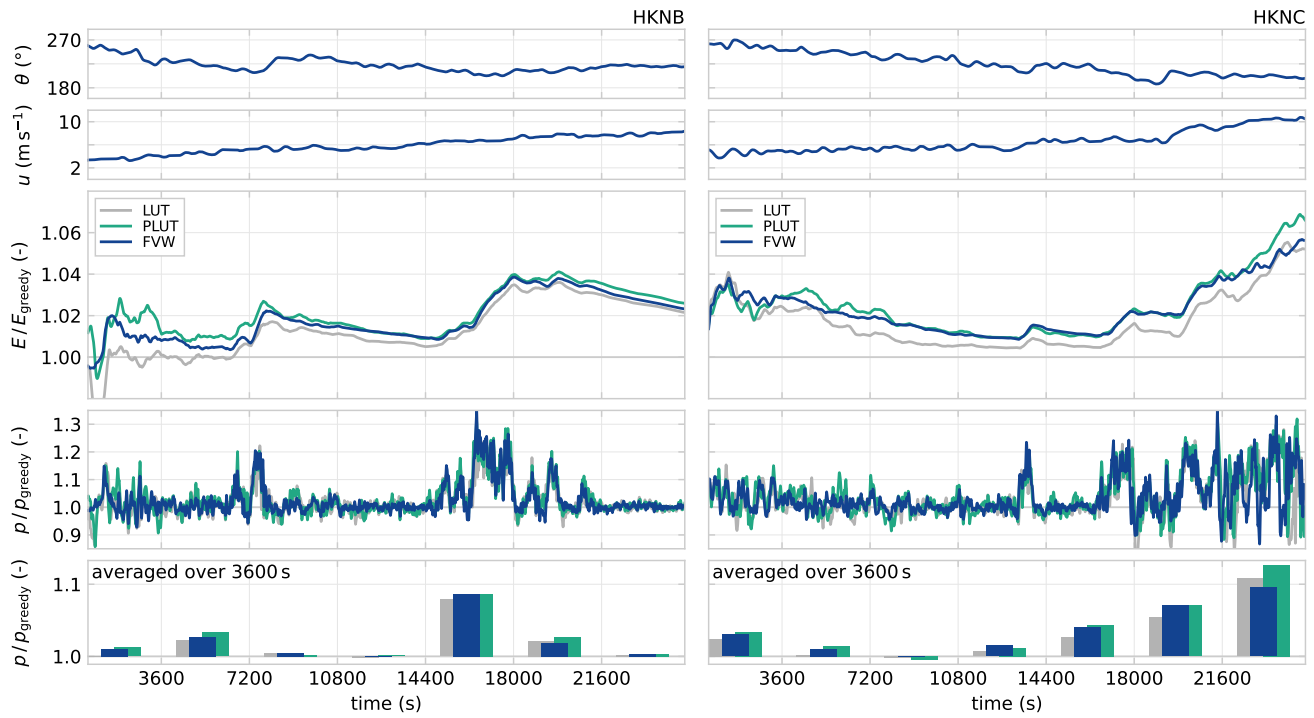
Figure 17. Relative energy produced, power over time, and power averaged in 3600s bins for the two data-driven test cases, HKNB and HKNC. The driving wind direction and wind speed are shown in the top two rows. The third row shows the cumulative energy time series normalised with respect to the greedy baseline controller. Both the LUT, PLUT, and the FVW controller exhibit significant improvements over greedy control. The bottom row shows the one-hour averaged power production of both controllers normalised by the greedy baseline.
