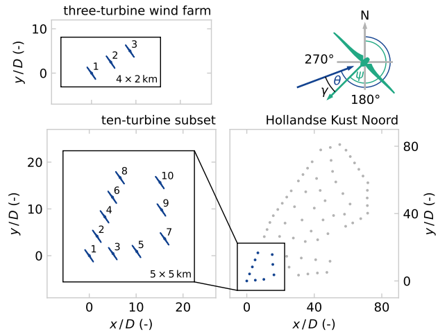
Figure 7. Layout of the wind farm test cases and simulation domains, and angle definitions for wind direction \theta , turbine heading \psi , and yaw misalignment \gamma = \theta - \psi . The three-turbine wind farm has a 5D spacing and is aligned along \theta = 240^\circ . The ten-turbine subset of Hollandse Kust Noord (HKN) is the South-West corner of the wind farm, scaled to the 10MW reference turbine.
