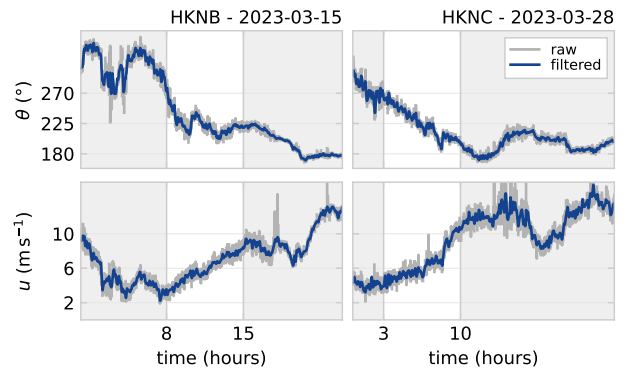
Figure 8. Time series of lidar measurements of wind direction and wind speed at the HKN location (KNMI, 2023). The raw data is post-processed and low-pass filtered with a [parse-numbers = false]1/600\text{ Hz} cut-off frequency. Two seven-hour time series with wind direction 180^\circ \leq \theta \leq 270^\circ and below-rated wind speeds are selected for driving the realistic wind variations in the LES.
