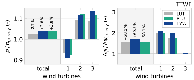
Figure 11. Cumulative results for the three-turbine test case in terms of total relative power production and yaw travel. The FVW controller improved power production at a slight increase in yaw travel compared to the LUT controller. In this case, the PLUT achieves the same improvement in power production as the FVW.
