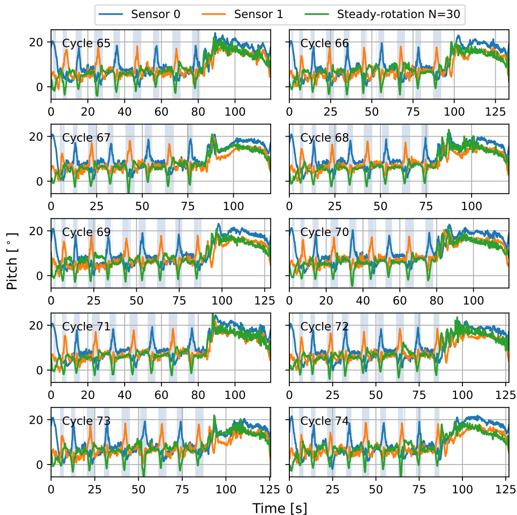
Figure 15. The pitch of the kite element with respect to the tangential plane along ten pumping cycles resulting from the steady-rotation-state analysis using 30 tether elements (T-I N=30), together with the kite pitch inferred from the wing attitude measured with two sensors. The shaded intervals indicate the turns during the reel-out phase. After the turns, the system transitions into the reel-in phase.
