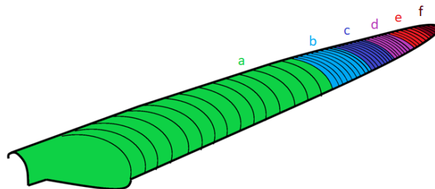
Figure 4. Blade sections and erosion securities introduced to the sections in terms of lift-to-drag losses. ('f' is the most severe erosion and 'a' is the clean case with no loss)
