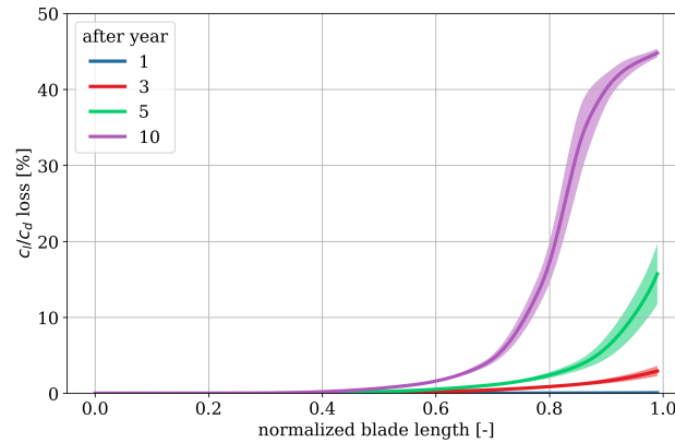
Figure 8. Snapshots of the wind farm-average lift-over-drag losses along the blade after 1, 3, 5 and 10 years of operation.
