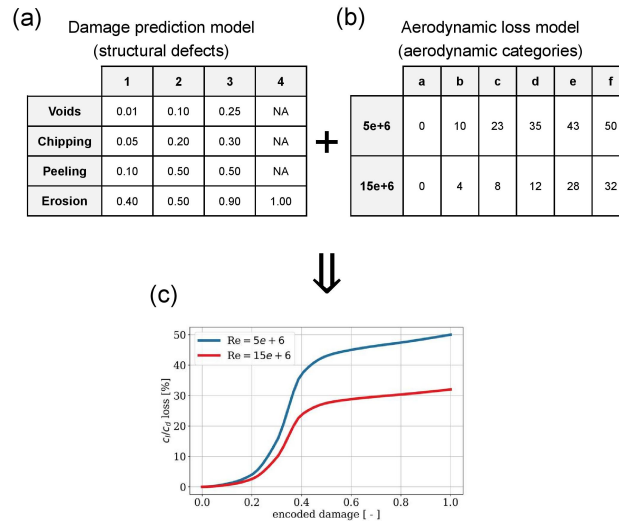
Figure 3. Mapping between aerodynamic loss and encoded structural defects. (a) shows the structural categories and associated encoded damage level, (b) shows the aerodynamic categories and associated lift-to-drag loss and (c) shows final coupling between the encoded damage level and aerodynamic loss.
