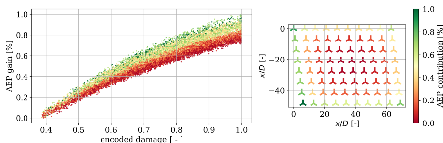
Figure 12. AEP gain plotted against the damage level of the repaired turbine. The colors indicate the reference AEP contribution which is also shown on the right-side figure. Both the AEP gain and reference AEP has been linearly normalized.
