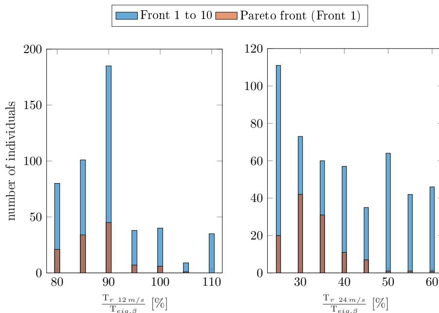
Figure 13. Controller decision space on the Pareto surface.
