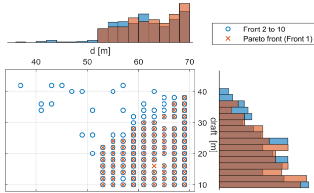
Figure 11. Geometric decision space on the Pareto surface.
