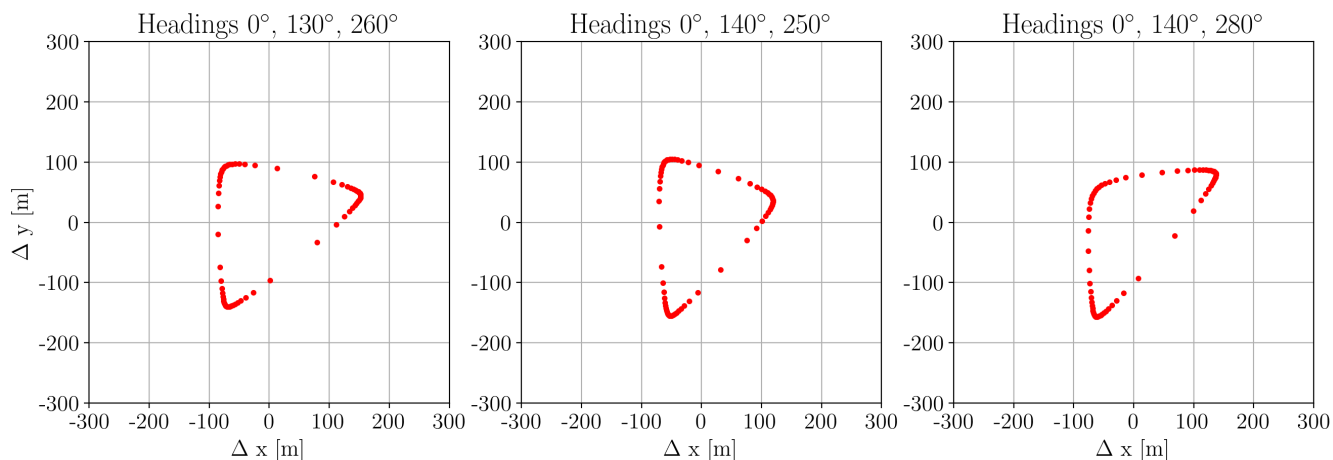
Figure 6. Three watch circles with three different mooring lines headings
