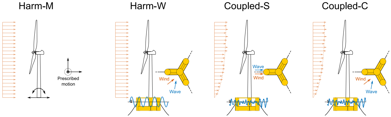
Figure 1. The influence of platform motion due to waves on the power production of floating wind turbines is studied with four simulation scenarios/models. In the Harm-M ease model , sinusoidal motion of varying amplitude and frequency is prescribed at the wind turbine tower base. In the Harm-W simulations model , the turbine is excited with regular waves of different amplitudes, frequencies and directions. In the coupled-simulations Coupled-S and Coupled-C models , the wind turbine response is computed for several environmental conditions with full-field turbulent wind and irregular waves; wind-wave conditions are obtained with simplifications typically used by standards (Coupled-S) or they are extracted by means of clustering from a database of met-ocean data (Coupled-C).
