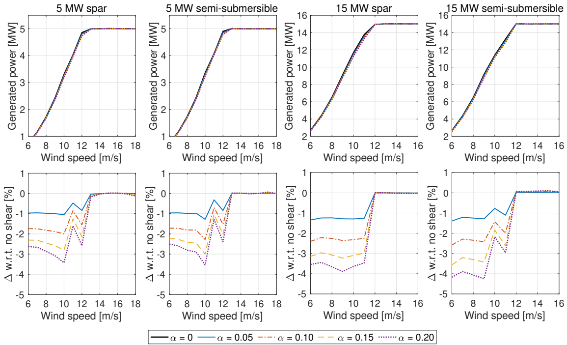
Figure 8. Sensitivity to Effect of wind shear of the four floating wind turbines. Power curves and percent variation of the power curve with respect to the case with no shear ( \alpha = 0 ).
