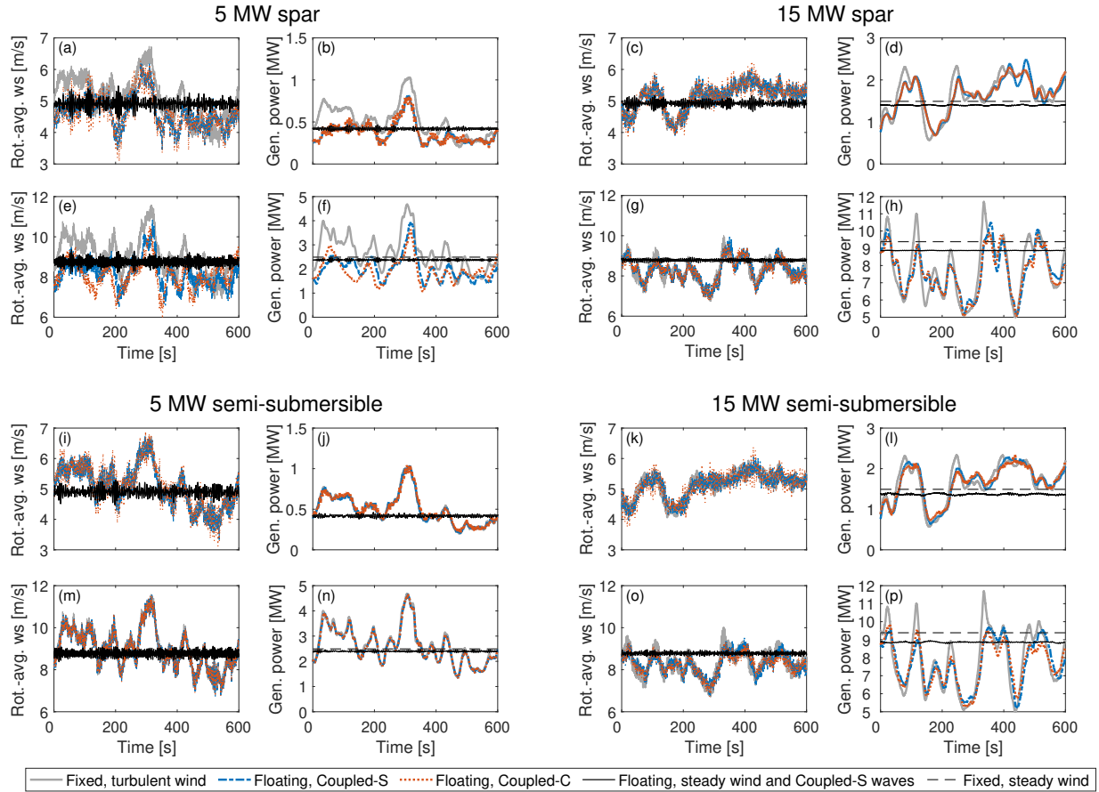
Figure 16. Effect of wind turbulence and waves on the power conversion process of the four floating wind turbines: time series of rotor-averaged wind speed and generated power. (a), (b), (c), (d), (i), (j), (k), (l) mean wind speed of 5 m/s. (e), (f), (g), (h), (m), (n), (o), (p) mean wind speed of 9 m/s.
