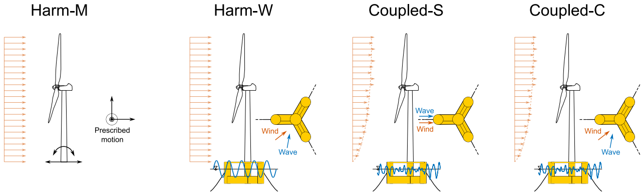
Figure 1. The influence of platform motion due to waves on the power production of floating wind turbines is studied with four simulation scenarios/models. In the Harm-M case/model, sinusoidal motion of varying amplitude and frequency is prescribed at the wind turbine tower base. In the Harm-W simulation/model, the turbine is excited with regular waves of different amplitudes, frequencies and directions. In the coupled-simulations/Coupled-S and Coupled-C models, the wind turbine response is computed for several environmental conditions with full-field turbulent wind and irregular waves; wind-wave conditions are obtained with simplifications typically used by standards (Coupled-S) or they are extracted by means of clustering from a database of met-ocean data (Coupled-C).
