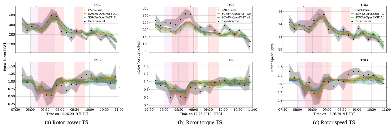
Figure 6. Time series results for rotor power, torque, and speed for all computational methods and experimental results (not SCADA). The subplots on the top are dimensional for Tr02 and on the bottom are non-dimensionalized for Tr03. Dots show 10 minute averages and bands extend to \pm 1 standard deviation from the mean. Results from each wind turbine are shown in separate sub-figures. Vertical shaded regions are used to show when wake steering of more than \pm 10^\circ is present (red) and when there was prominent wakening of Tr03 and Tr04 (purple).
