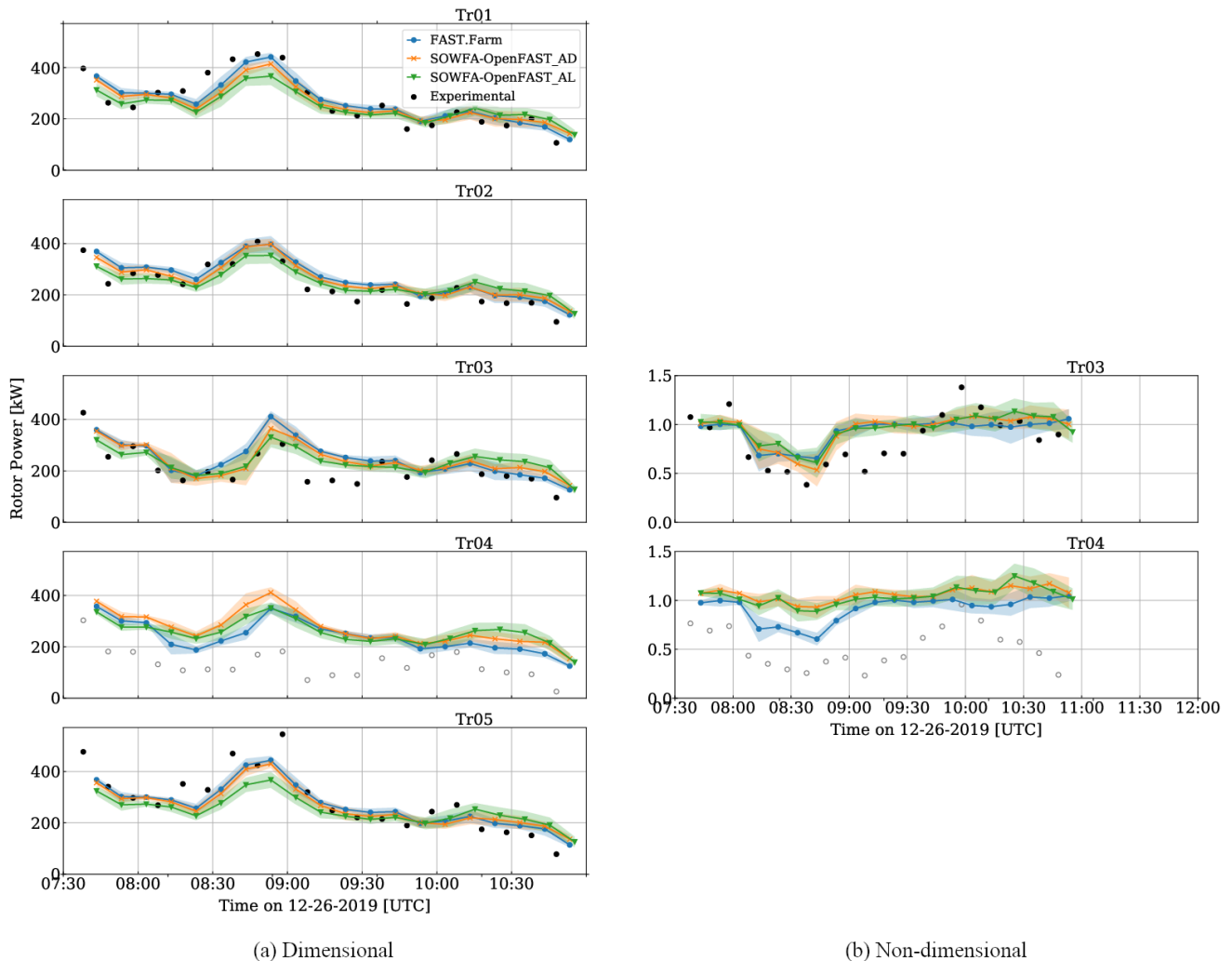
Figure 5. Time-series (TS) results for rotor power of all turbines for all computational methods and experimental results. The subplots on the left (a) are dimensional and on the right (b) are non-dimensionalized. Dots show 10 minute averages and bands extend to \pm 1 standard deviation from the mean. Results from each wind turbine are shown in separate sub-figures. Experimental results for Tr04 are invalid.
