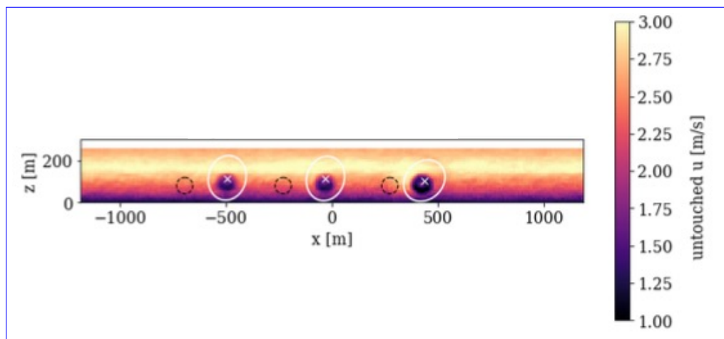
Figure 4. Instantaneous snapshot of FAST.Farm u-velocity located 2D downstream of Tr01, Tr02, and Tr05. Black circles show the projected location of the rotor plane. White circles show the area searched for calculating the wake center of the corresponding wind turbine wake, with the white x showing the calculated instantaneous wake center location at 1 hour into the simulation.
