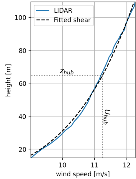
Figure 9. Measured wind shear profile from LIDAR for Scenario 1 (Case 1 and 2).
