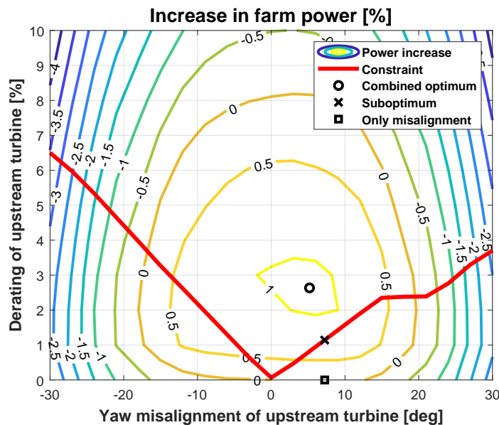
Figure 9. Contour plot of the overall power output of the two-turbine farm with s = 3D , y_h = 0 and at V = 11.4\text{m/s} and \text{TI} = 6\% . The red solid line represents the overall constraint function. Optimal control set-points are also visualized as a square marker (reference wake redirection, only misalignment), circle marker (combined and constrained control), and \times marker (sub-optimal control).
