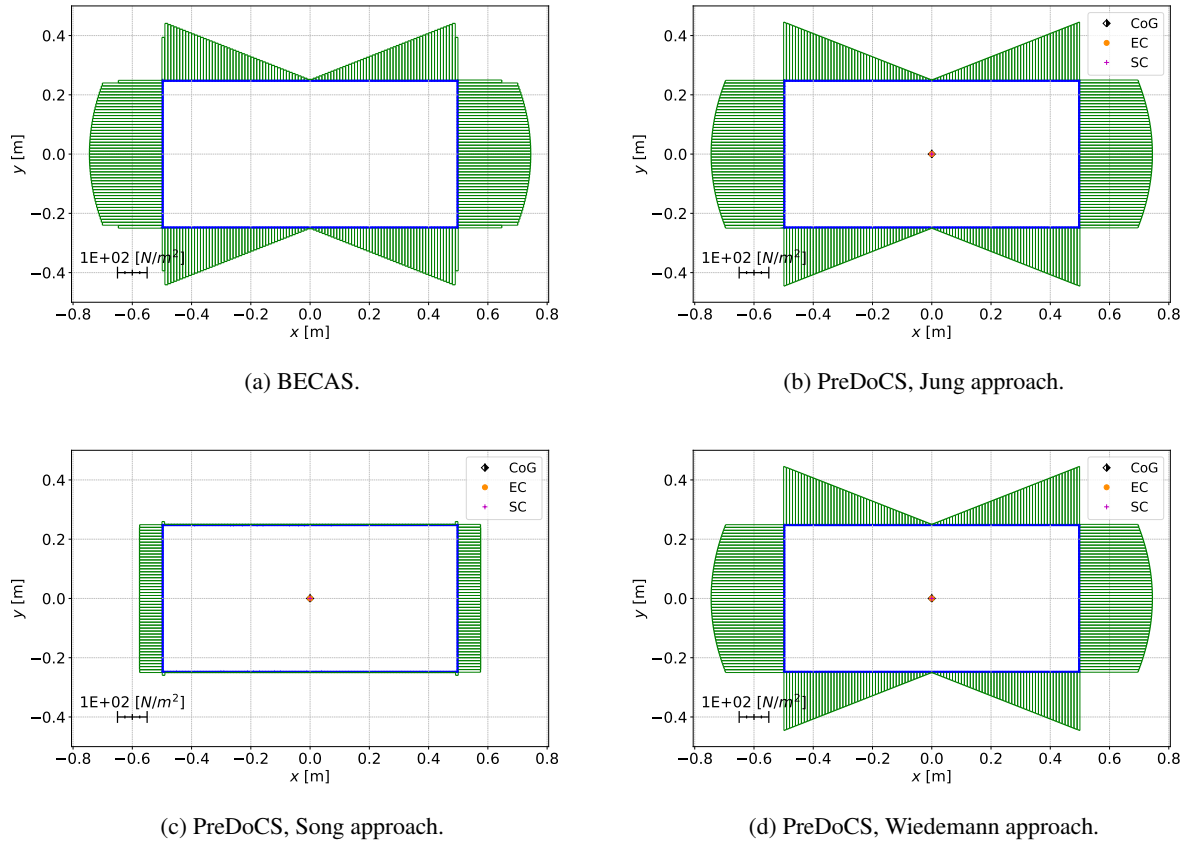
Figure 5. Shear stress \sigma_{zs} distribution for test case 0 under a unit transverse force in y -direction.
