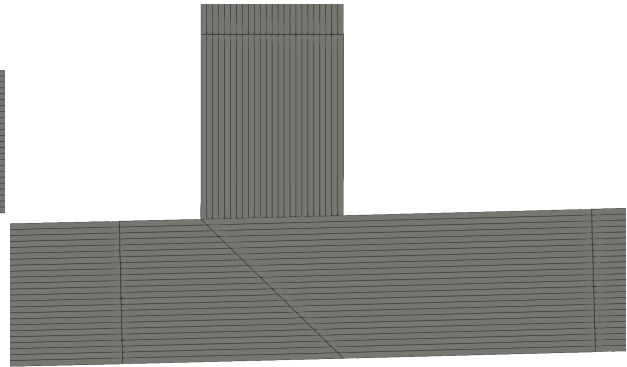
(d) Test case 11 (BECAS), close-up of the front lower web-shell-intersection.
