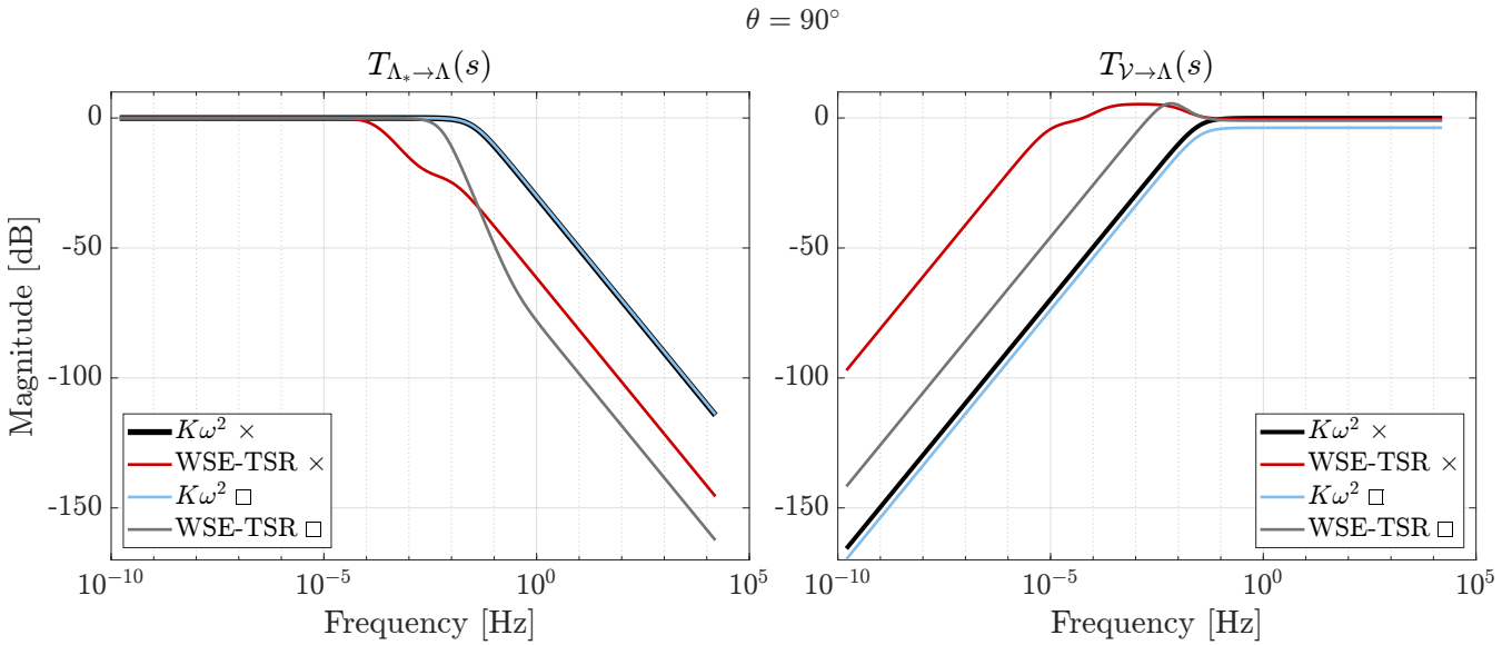
Figure 13. Bode plots of the closed-loop transfer functions T_{\Lambda_* \rightarrow \Lambda}(s) and T_{\gamma \rightarrow \Lambda}(s) for the baseline K\omega^2 and the WSE-TSR tracking controllers. The MCDM solutions for the WSE-TSR tracking controller reveal that the reference tip-speed ratio tracking and disturbance rejection capabilities have to be offset to achieve 39% increase in power production, for the case \times , and 25% reduction in actuation effort, at the cost of 2% power decrease and 6% increase in psychoacoustic annoyance, for the case \square , compared to the K\omega^2 controller.
