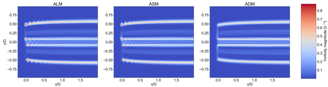
Figure 21. Vorticity magnitude along the streamwise direction for ALM, ASM, ADM, respectively from left to right. Fine mesh with \frac{D}{\Delta x_{min}} = 64 .
