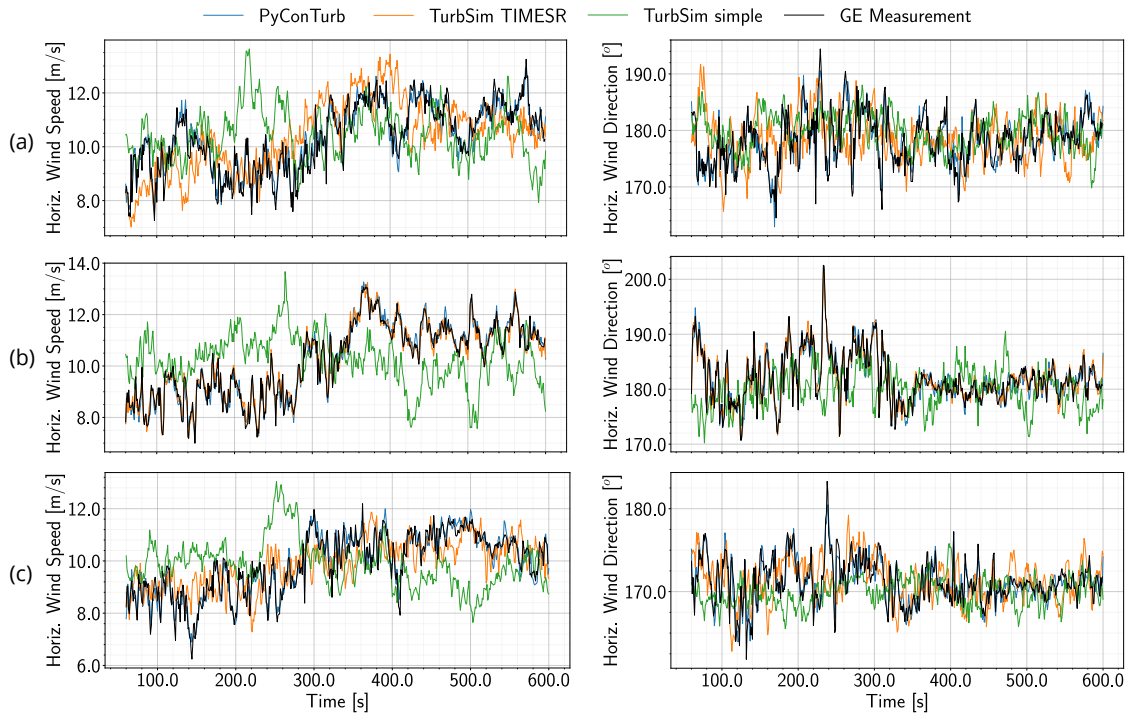
Figure 8. Comparison of time series of simulated inflow to measured inflow for a sample an example 10-minute bin for the sonic anemometers near (a) top tip, (b) hub height, and (c) bottom tip. The simulated data have been interpolated from the computational grid to the exact measurement locations, which were 179.5 m, 110.5 m, and 52.6 m, respectively. Only one of six turbulence seeds is shown.
