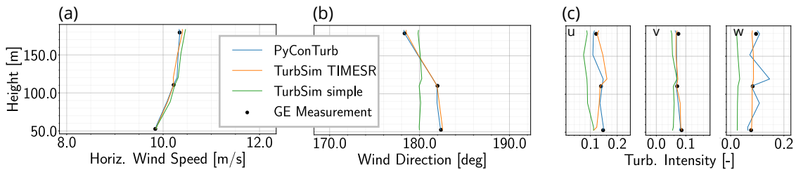
Figure 10. Comparison of vertical profiles of simulated inflow to measured inflow for a sample an example 10-minute bin for (a) horizontal wind speed and (b) direction, and (c) the three components of turbulence intensity, which are calculated as the standard deviation of the given component divided by the mean of the u component. Only one of six turbulence seeds is shown.
