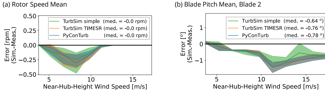
Figure 13. Comparison of (a) mean rotor speed and (b) mean blade pitch between models and measurement. The plots consist of statistics of calculated within each wind speed bin wind speed interval including the median (solid lines) and interquartile range (shaded areas). The median value reported in the legend is the overall median error calculated across all 10-minute bins.
