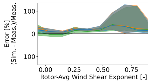
(b) Near-Root Flapwise Moment DEL, Blade 1 (vs. Wind Shear Exp.)
