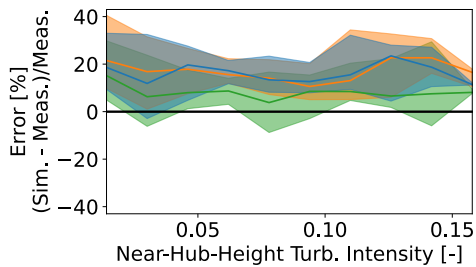
(a) Near-Root Flapwise Moment DEL, Blade 1 (vs. Turb. Intensity)
