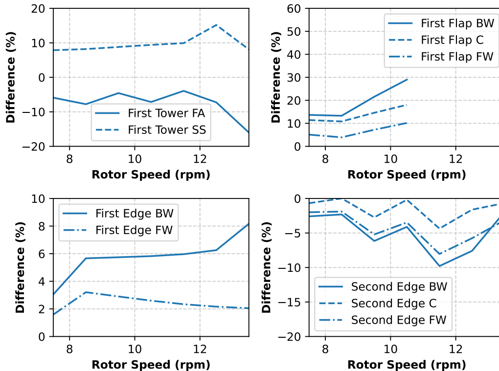
Figure 3. Relative differences between numerical (OpenFAST) and experimental (from blade-root strain gauges) natural frequencies for first tower modes (top left), first rotor flap modes (top right), first rotor edge modes (bottom left), and second rotor edge modes (bottom right). For the tower, fore-aft (FA) and side-side (SS) modes are reported. For the rotor, backward whirling (BW), collective (C), and forward whirling (FW) modes are reported. Positive values represent higher frequencies in OpenFAST relative to experimental values.
