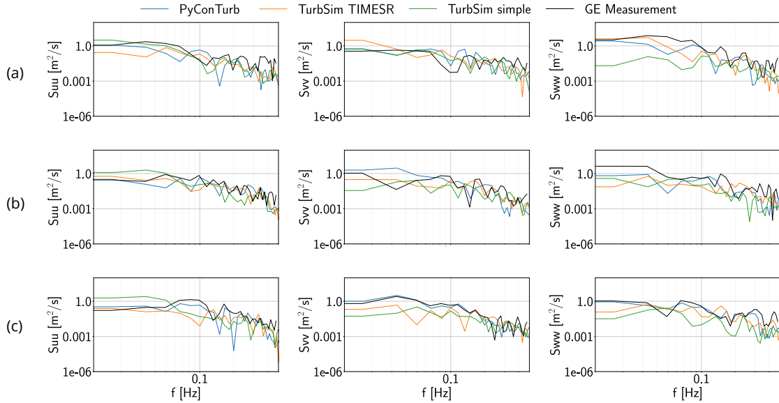
Figure 9. Comparison of turbulence spectra of simulated inflow to measured inflow for a sample an example 10-minute bin for the sonic anemometers near (a) top tip, (b) hub height, and (c) bottom tip. Before calculating the spectra, the simulated data have been interpolated from the computational grid to the exact measurement locations, which are 179.5 m, 110.5 m, and 52.6 m, respectively. Spectra are calculated with the one-sided welch method using 60 s bins and a Hanning window. Only one of six turbulence seeds is shown.
