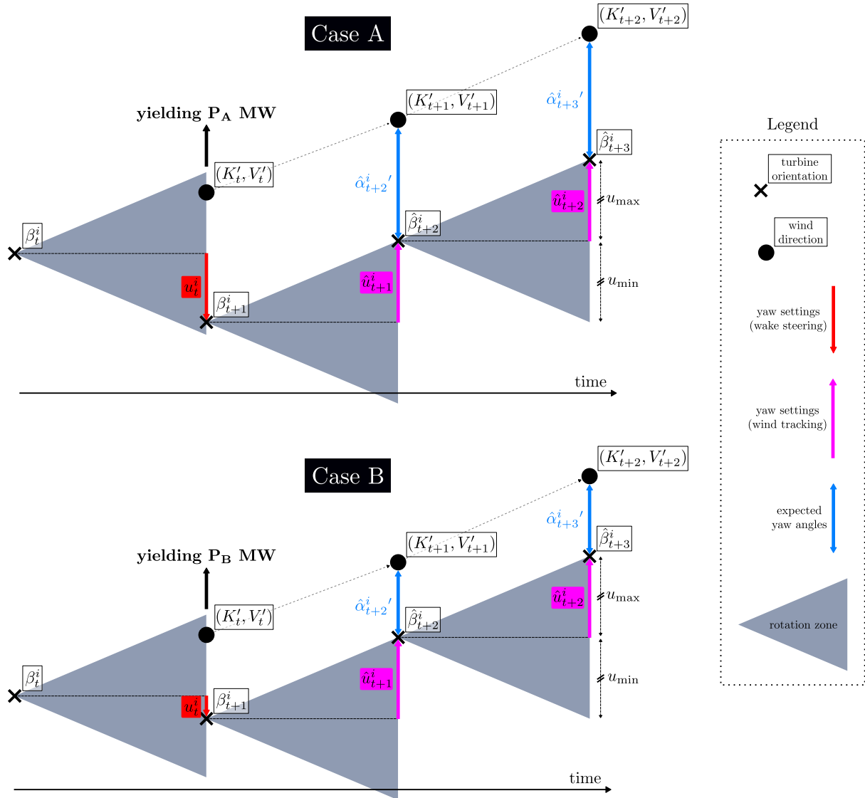
Figure 3. Illustration of the heuristic for a turbine i at time step t for two different cases. The horizon is L = 2 and the wind data is the same for cases A and B. Wake steering optimization is performed to find the setting u_t^i , which yields a power output of P_A MW for case A and P_B MW for case B at time step t . By considering P_A > P_B , the case A would be preferred. But the heuristic computes the future expected yaw angles, if a naive wind tracking solution is used, to get an average idea of how far the turbine will be from the predicted wind direction. Here, while the yaw setting of case A gives a better immediate solution than the one given by case B, it keeps the turbine further away from the future wind. The solution of case B would then be preferable. The heuristic encourages the choice of yaw settings that may not be the best at the current time step but that ensure future power output.
