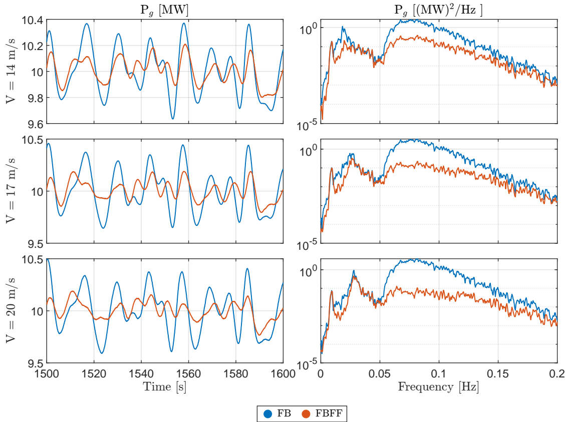
Figure 20. Generator power response with and without wave feedforward control, at different steady wind speeds at 14 m/s, 17 m/s and 20 m/s, and long-crested waves with H_s = 7 m, T_p = 12 s, and S = \infty .
