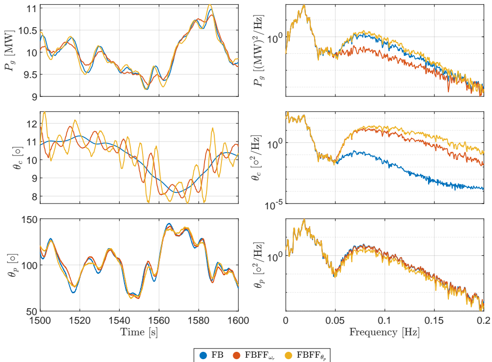
Figure 8. Generator power ( P_g ), blade pitch ( \theta_c ) and platform pitch ( \theta_p ) responses with and without wave feedforward control, at wind V = 14 m/s, TI = 7.1\% , and wave conditions of H_s = 5 m and T_p = 12 s. The two feedforward controllers, for the objectives of power regulation and platform pitch motion reduction are compared to the baseline feedback controller.
