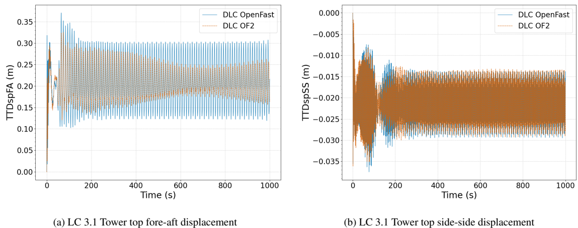
Figure 11. Tower top deformations for the regular wave case, LC 3.1. Tower top fore-aft deflection (left) and tower top side-side deflection (right). The results obtained with OpenFAST have been presented in blue while OF 2 have been represented in orange.
