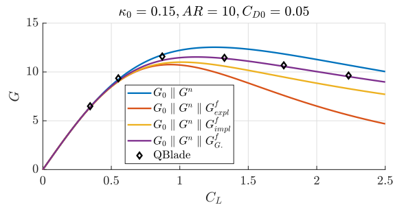
Figure B4. Glide ratio as function of the lift coefficient for a case with \mathcal{R} = 10 , \kappa_0 = 0.15 and C_{D0} = 0.05 .
