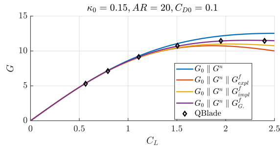
Figure B1. Glide ratio as function of the lift coefficient for a case with \mathcal{R} = 20 , \kappa_0 = 0.15 and C_{D0} = 0.1 .
