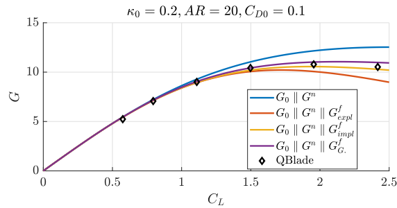
Figure B3. Glide ratio as function of the lift coefficient for a case with \mathcal{R} = 20 , \kappa_0 = 0.2 and C_{D0} = 0.1 .
