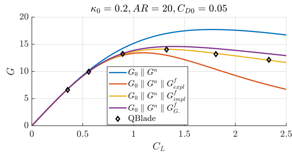
Figure B2. Glide ratio as function of the lift coefficient for a case with \mathcal{R} = 20 , \kappa_0 = 0.2 and C_{D0} = 0.05 .
