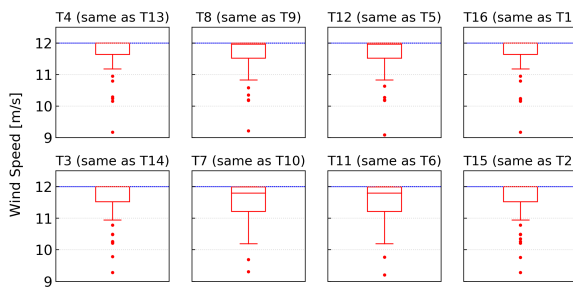
(b) Near-rated scenario
