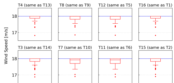
(c) Above-rated scenario
