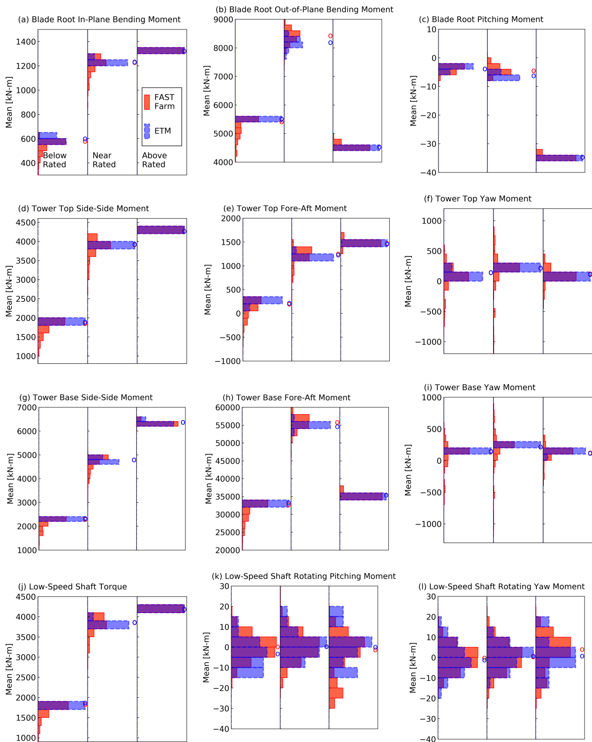
Figure 17. Distribution of 10-minute means ( \mu ) for loads. Each subpanel gives the distributions for FAST.Farm (11,520 points: 16 wind turbines, 10 seeds, 72 wind directions) and the effective turbulence model (160 points: 16 wind turbines, 10 seeds).
