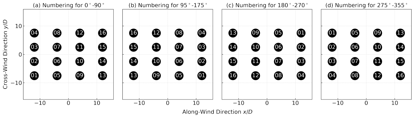
Figure 3. Wind turbine mapping used to broadcast the 19 simulation results spanning 0^\circ – 90^\circ to the other three quadrants.
