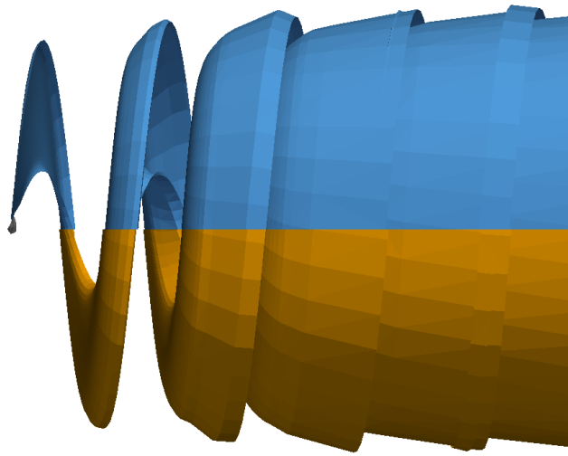
Figure 27. Wake for real (top, blue) and pseudo (bottom, orange) surge motion at f = 1 Hz. Only one blade shown.
