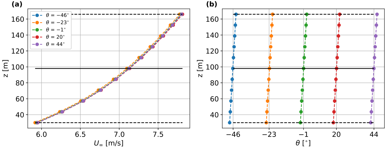
Figure 2. Vertical profiles of the horizontal wind speed (a) and wind direction (b) extracted at the location of T92 from the freestream simulations. Black lines indicate hub height (continuous) and rotor tips (dashed).
