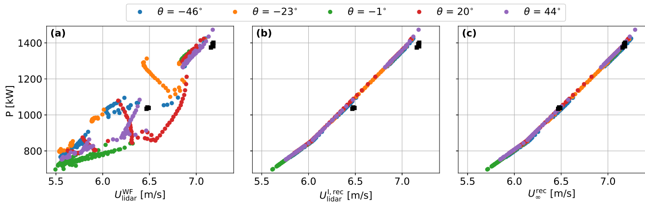
Figure 10. Power output against the lidar-measured wind speed of all the wind-farm turbines for all wind directions. (a): no correction applied on the measured wind speed. (b): wind speed corrected with Eq. (1). (c): wind speed corrected with Eq. (2). Black squares indicate points with the combination ( U_\infty, P^I ) from the isolated and freestream simulations.
