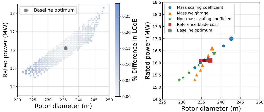
Figure 9. (a) Sensitivity of the optimum design to rotor model parameters for random combinations of parameter values. (b) One-at-a-time variation per parameter (the larger markers correspond to the lower end of the parameter variation range).
