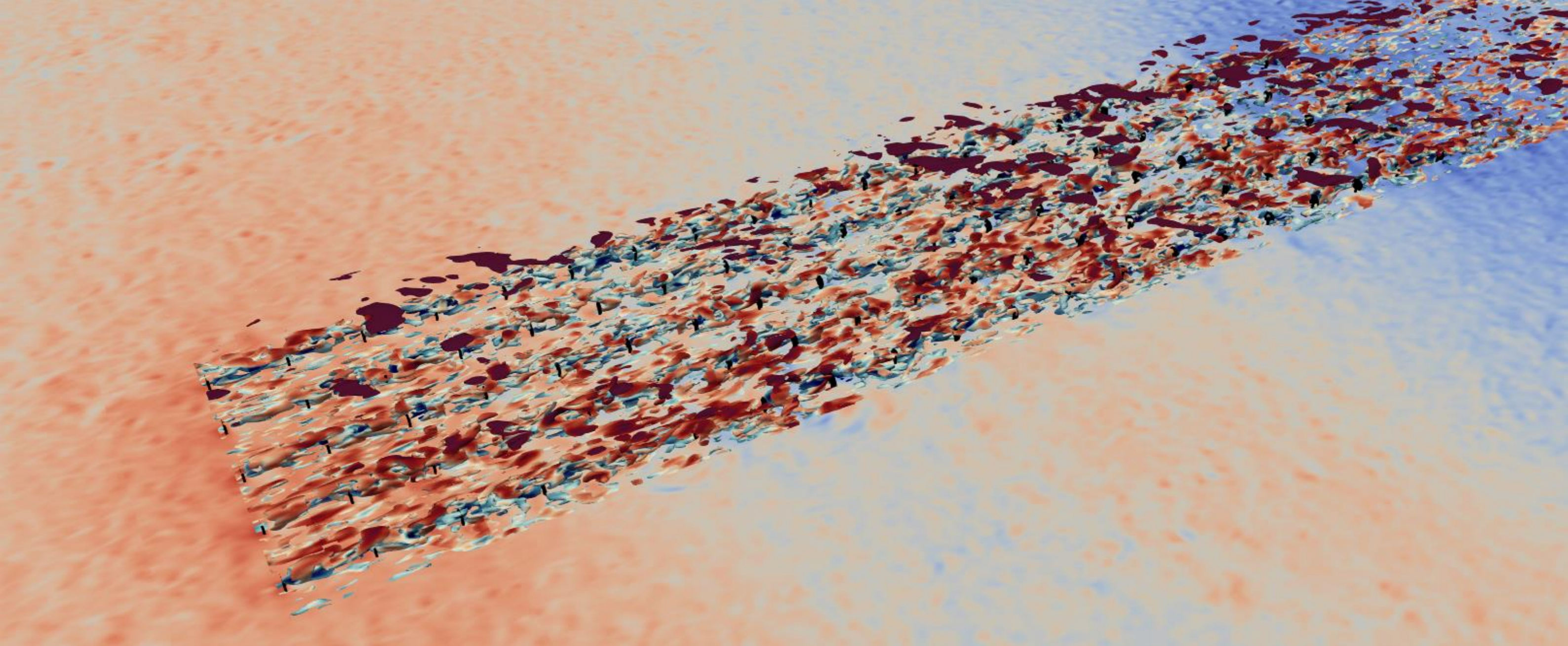
Q-criterion iso-surfaces at level 0.007, and wind farm-induced gravity wave signature visualized as background pressure perturbations on a slice at the hub-height.
