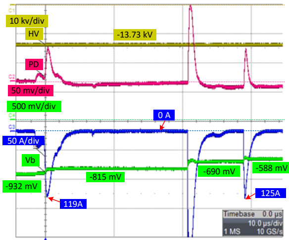
275 Figure 21: Bearing voltage and current at -13.73 kV needle voltage.
