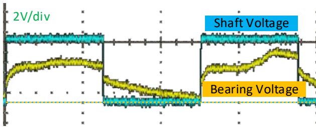
Figure 17: Bearing voltage without grease.
