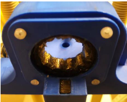
Figure 13: Cylindrical roller bearing (in housing) packed with extra lubrication grease.
