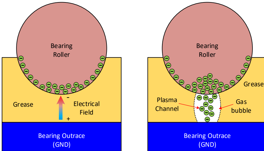
Figure 23: Charge movement during breakdown.
