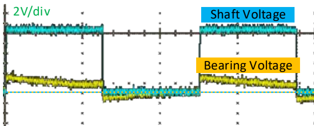
245 Figure 18: Bearing voltage with grease.
