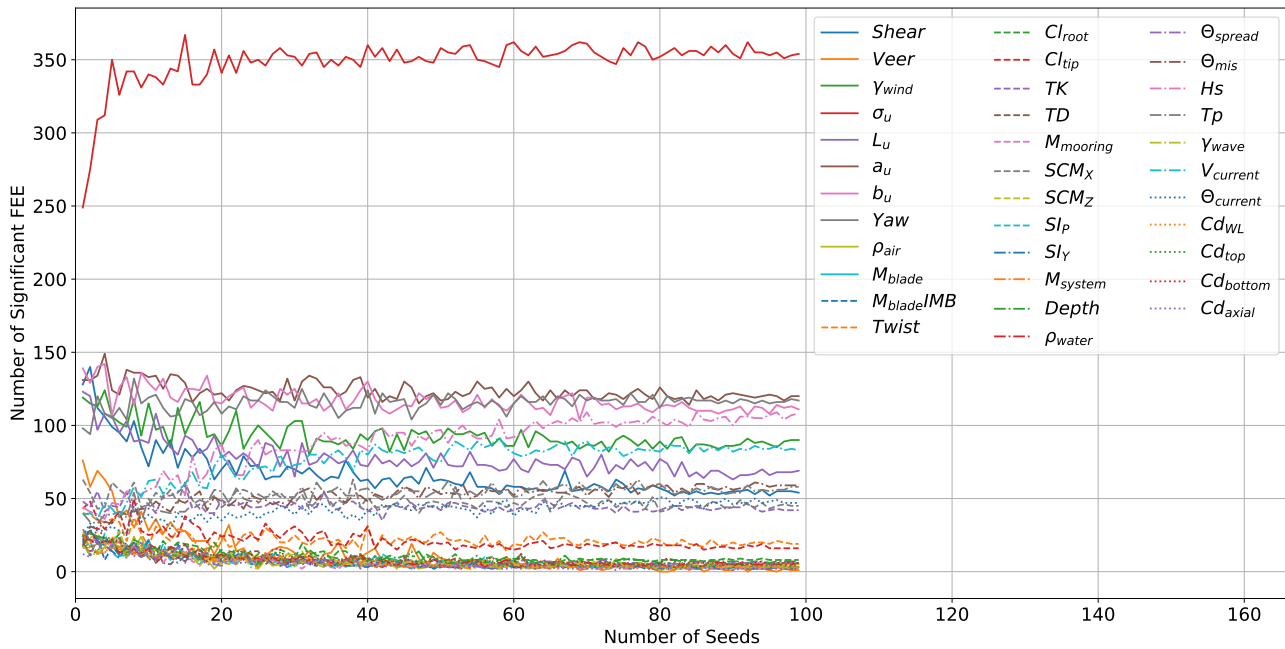
Figure 9. Convergence of fatigue response sensitivity due to number of random seeds
