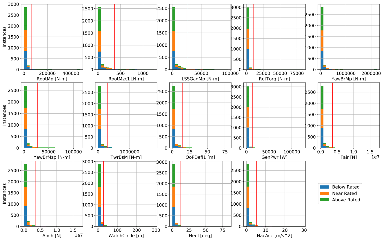
Figure 5. Fatigue EE value histograms broken by wind speed condition for 14 quantities of interest; red line marks threshold for significant EE value
