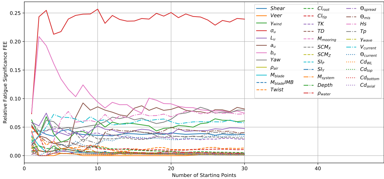
Figure 11. Convergence of fatigue response sensitivity due to number of input parameter hyperspace starting points
