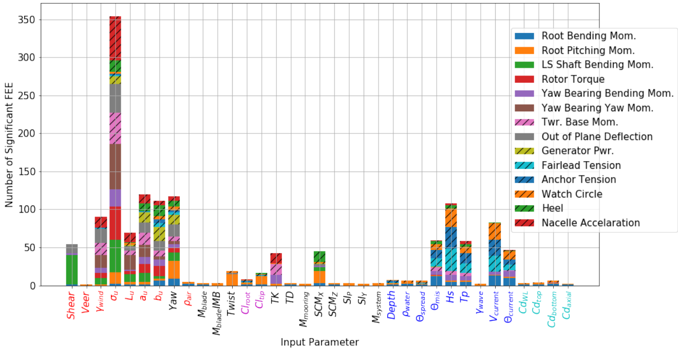
Figure 7. Floating offshore wind turbine fatigue load EE sensitivity, broken by load type, solid bars correspond to turbine specific responses and hatched bars correspond to global system responses (input parameter colors: red = inflow wind, magenta = aerodynamic forces, black = system and structure, blue = sea state, and cyan = hydrodynamic forces)
