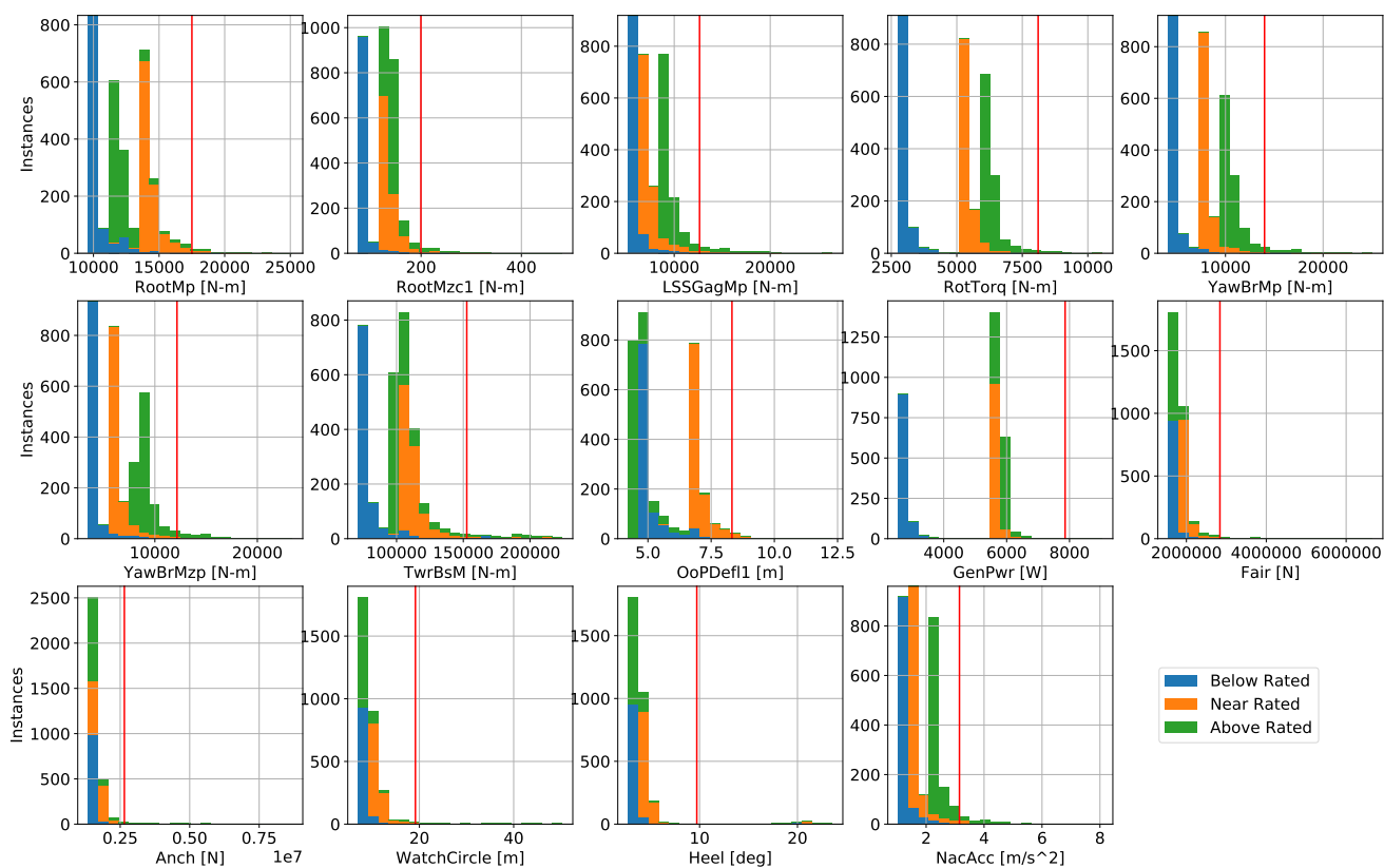
Figure 4. Ultimate EE value histograms broken by wind speed condition for 14 quantities of interest; red line marks threshold for significant EE value
