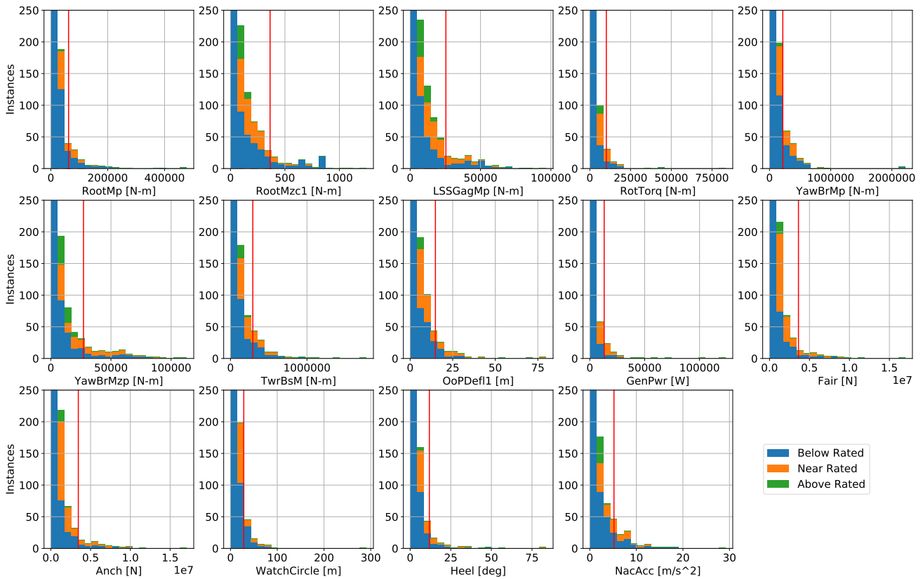
Figure A1. Fatigue EE value histograms broken by wind speed condition for 14 quantities of interest with a zoomed y-axis ; red line marks threshold for significant EE value
