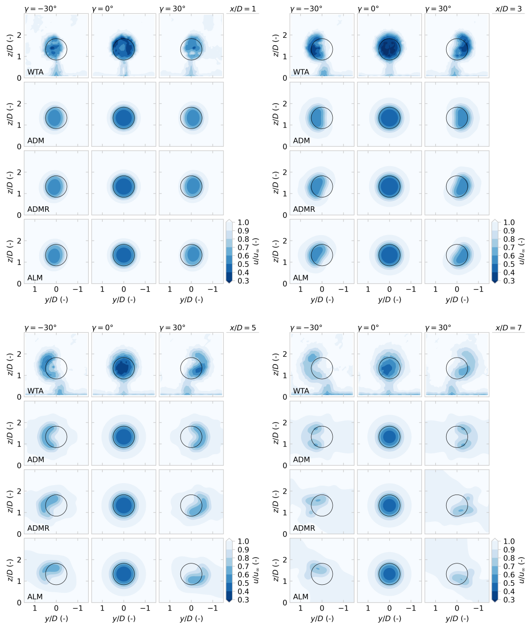
Figure 8. A comparison of normalised streamwise velocity for wind turbines under yaw misalignment. The experimental data from WTA are compared to model results with the ADM, ADMR, and ALM with slices at x/D = \{1, 3, 5, 7\} for yaw misalignment angles \gamma = \{-30^\circ, 0^\circ, 30^\circ\} . All three models represent the curled shape of the wake under yaw misalignment. The inclusion of rotation (ADMR, ALM) improves the qualitative representation of the asymmetry and vertical displacement that is observed in the wind tunnel. The deformation of the vortex filament structure with the ALM beyond x/D = 5 becomes too large to provide useful predictions.
