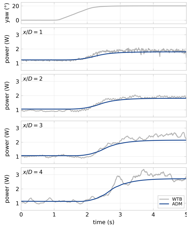
Figure 11. The realisation of the \gamma = 20^\circ step in yaw angle measured in WTB is shown in the top graph. The rotor-averaged potential power is calculated directly downstream of the turbine from for x/D = \{1, 2, 3, 4\} , comparing the experimental data and a simulation with the ADM. The FVW implementation of the ADM follows the dynamics of wake redirection well and estimates a potential power improvement of similar magnitude, although it lacks the turbulent disturbances.
