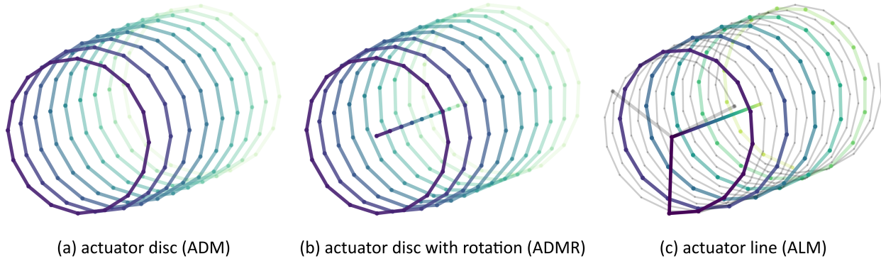
Figure 1. The vortex filament structures for the three different free-vortex wind turbine representations under consideration: (a) the actuator disc (ADM) builds up a wake with discretised vortex rings, (b) the actuator disc with rotation (ADMR) adds a root vortex along the wake centre to model swirl due to turbine rotation, and (c) the actuator line (ALM) models individual blade circulation, tip vortices, and a combined root vortex. In (c), the vortex structure from a single blade is highlighted for clarity.
