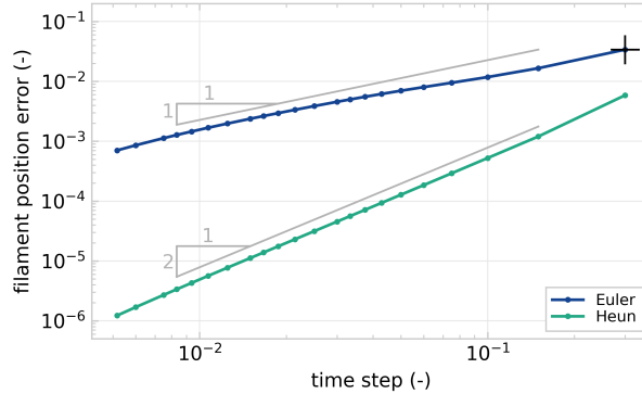
Figure 3. Relative error of the position of the vortex filaments for varying time discretisation, comparing the first order explicit Euler method and the second order explicit Heun’s method. Reference solution for time step \Delta t \cdot u_\infty / D = 1.5 \times 10^{-3} . The cross ‘+’ marks \Delta t \cdot u_\infty / D = 0.3 as used throughout this paper.
