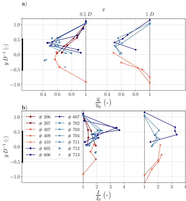
Figure 12. a) Lateral profile of normalized wind speed \bar{u}/\bar{u}_0 in the WT wake at different downstream distances ( x = 0.5 D and 1 D ). b) Lateral profile of normalized turbulence intensity I/I_0 at the bottom figure. Different colors indicating different flight days. The blue color represents stable to near-neutral atmospheric conditions while the red color indicates unstable convective conditions (dark red for highly unstable and light red for less unstable cases).
