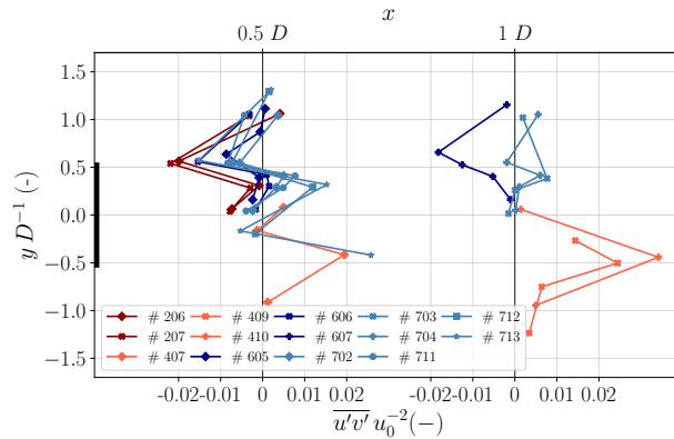
Figure 14. Lateral profile of normalized horizontal fluxes \overline{u'v'}/\overline{u_0^2} in the WT wake at different downstream distances ( x = 0.5 D and 1 D ). Different colors indicate different flight days. Blue represents stable to near-neutral atmospheric conditions while red indicates unstable convective conditions.
