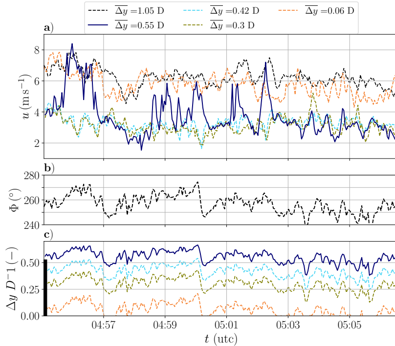
Figure 6. Time-series of wind velocity a), wind direction in b) and lateral position c) of a lateral flight pattern in stable conditions (fl. # 606). The lateral positions are calculated using the wind direction of reference UAS measurement, which is shown in the middle figure. The black bar in c) indicates the lateral position of the WT.
