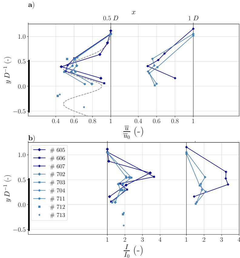
Figure 8. a) Lateral profile of normalized wind speed \bar{u}/\bar{u}_0 in the WT wake at different downstream distances ( x = 0.5 D and 1 D ). b) Lateral profile of normalized turbulence intensity I/I_0 at the bottom figure. Different colors indicating different flight days with both stable (dark blue) to near-neutral conditions (light blue). Details about the considered flights are found by the flight number in table 1. The grey dashed line indicating a mean double Gaussian symmetric fit of the present data.
