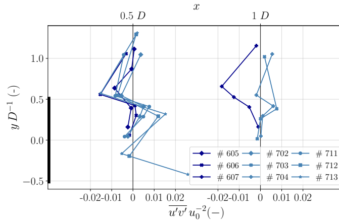
Figure 11. Lateral profile of normalized horizontal momentum fluxes \overline{u'v'}/\overline{u_0^2} in the WT wake at different downstream distances ( x = 0.5 D and 1 D ). Different colors indicating different flight days with both stable (dark blue) to near-neutral conditions (light blue).
