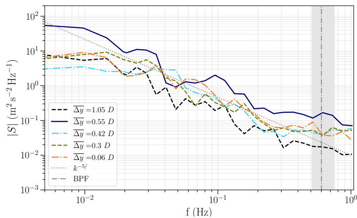
Figure 7. Power spectra of streamwise velocity S_u for flight # 606 (lateral pattern) at different lateral positions \Delta y . The blade-passing frequency (BPF) is indicated by the vertical dashed dotted line. The grey background around the BPF represents the bandwidth of the BPF based on the extremes of WT revolution speed. The spectra are processed with bin-averages in the frequency-space to decrease the noise.
