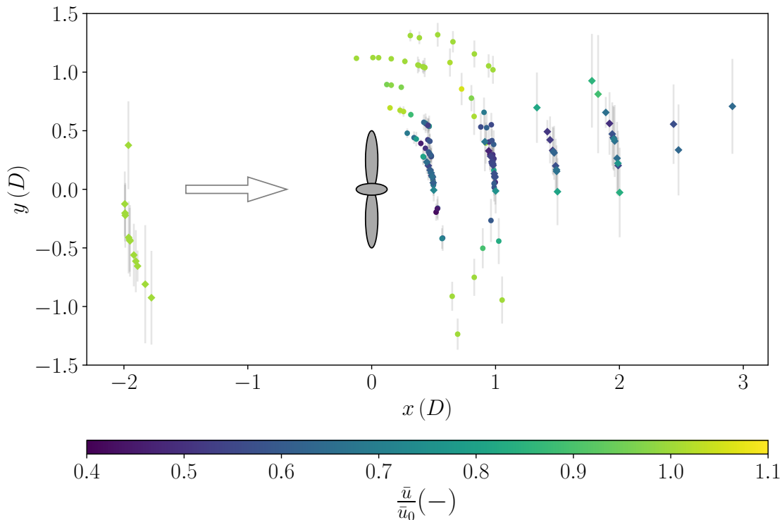
Figure 4. Normalized wind velocity of UAS measurements \bar{u}/\bar{u}_0 at locations relative to the reference wind direction. The black bar represents the position and dimensions of the WT rotor. Diamonds marker represent the longitudinal flight pattern while circle markers define the lateral flight pattern. The arrow indicates the inflow wind direction. The standard deviation in lateral position is illustrated by the grey vertical lines and is calculated from the standard deviation of the inflow wind direction.
