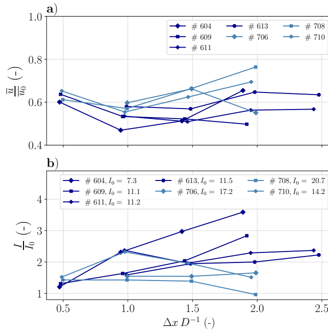
Figure 9. a) Normalized wind speed \bar{u}/\bar{u}_0 and b) normalized turbulence intensity I/I_0 is shown in the center of WT wake at different downstream distances. Different colors indicating different flight days with both stable (dark blue) to near-neutral conditions (light blue). The reference turbulent intensity I_0 given in the legend is shown in %.
