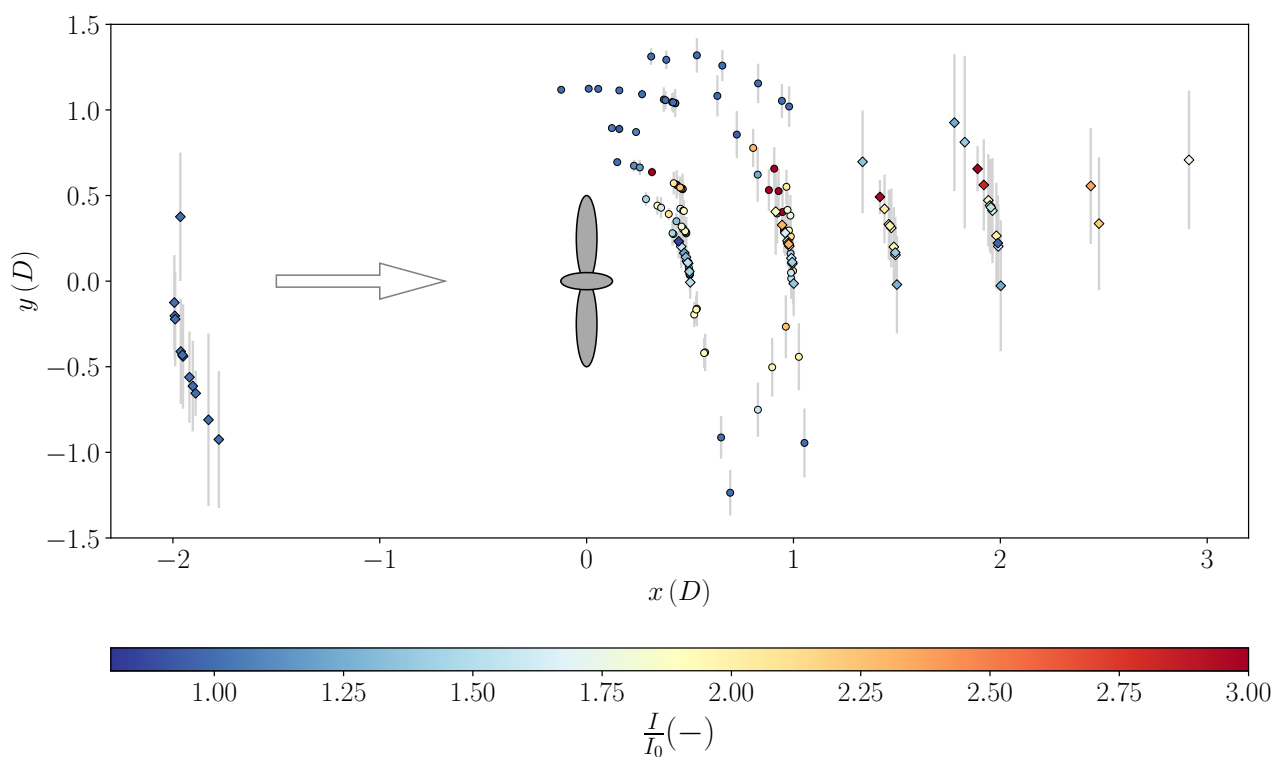
Figure A1. Normalized turbulence intensity I/I_0 of UAS measurements at locations relative to the reference wind direction.
