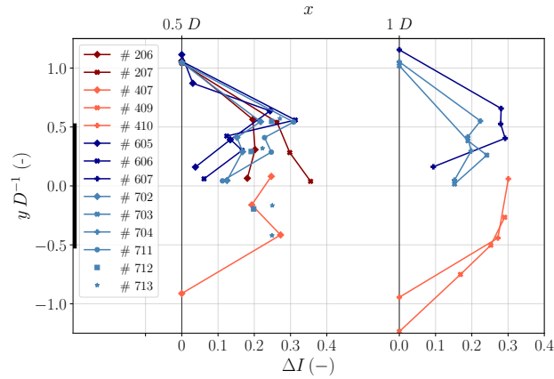
Figure 13. Lateral profile of added turbulence intensity \Delta I in the WT wake at different downstream distances ( x = 0.5 D and 1 D ). Different colors indicating different flight days. The blue days representing stable to near-neutral atmospheric conditions while the red days indicating unstable convective conditions.
