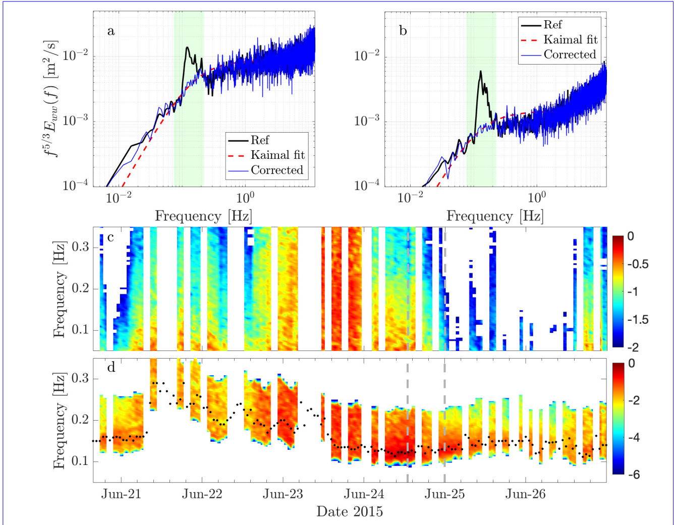
Figure 6. (a,b) Scaled power spectra of vertical velocity fluctuations w' for two events drawn as vertical grey dashed lines in Fig. 2a, and the corresponding corrected (decomposed) spectra (blue curves)). The red dashed lines show the spectral curves calculated from Eq. (6); and (c,d) energy-time spectra of decomposed vertical velocity w' and the wave-induced vertical velocity \tilde{w} fluctuations by the use of suggested decomposition algorithm. The black dotted markers in (d) are the wave peak frequency-frequencies extracted from buoy measurements.
