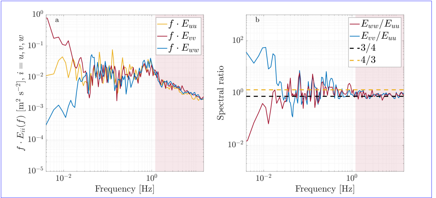
Figure A1. (a) Three-dimensional velocity spectra f \cdot E_{ii}(f) for i = u, v, and w (illustrated in Fig. 4d) showing the spectral regions of the wave-affected peaks and the inertial subrange; and (b) velocity spectra ratios with horizontal dashed yellow and black lines indicating the value of 4/3 and 3/4 , respectively.
