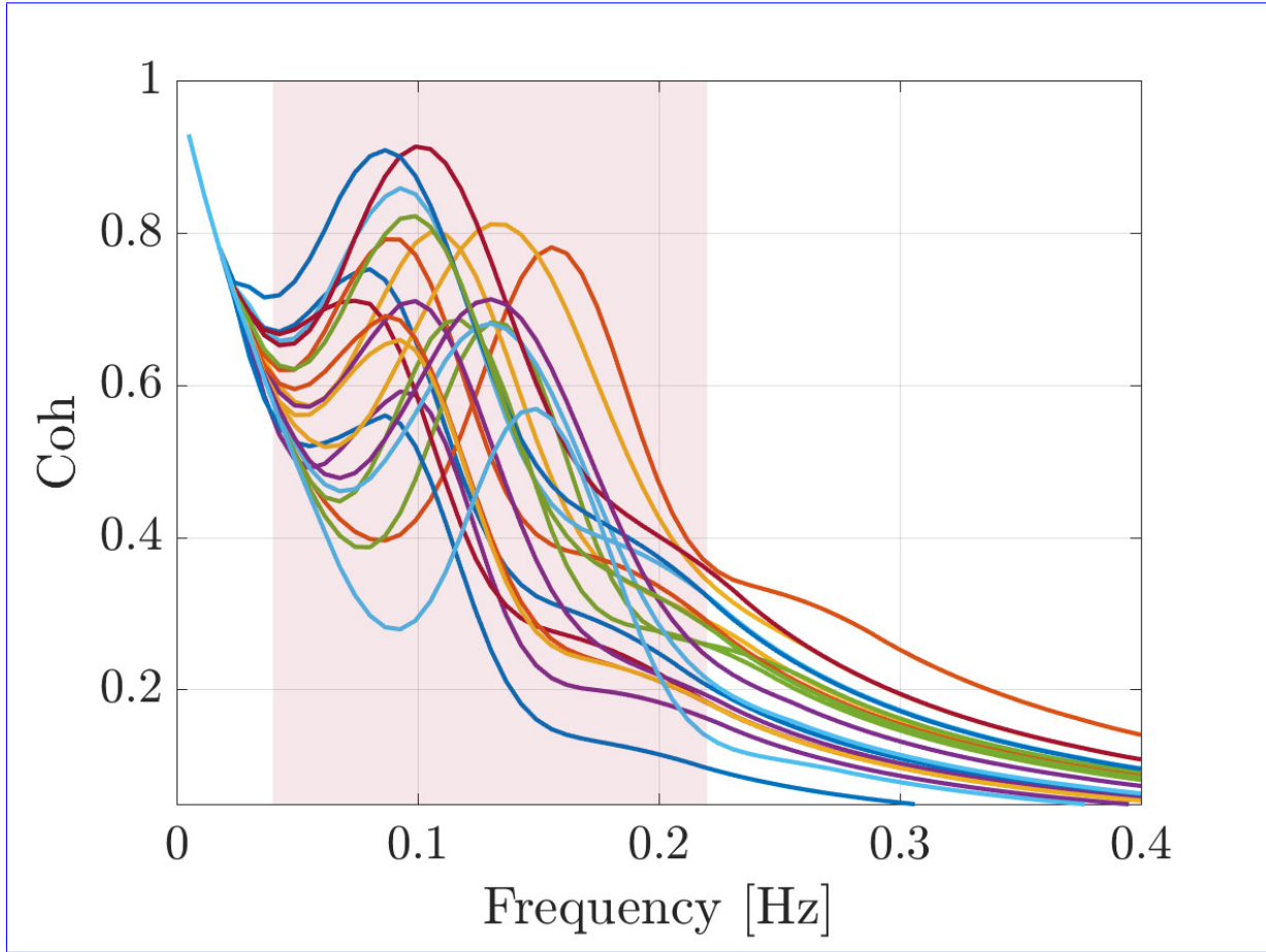
Figure B1. Theoretical coherences are generated based on the fundamental parameters listed in Table B1. To create 20 ensembles, we perturb H_s within the range of [0.5, 1.5], T_p within [5, 12], A_1 within [0.1, .5], and A_2 within [0.02, 0.1]. It's important to note that in the theoretical model defined in Eq. (2), we only use Term1 and Term2 to produce this figure.
