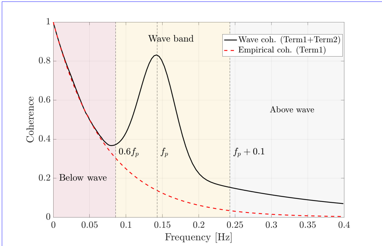
Figure 1. Comparing the coherence of the vertical velocity component of wind turbulence using the Davenport empirical model (Term1) to the wind-wave coherence (depicted by the black line) as shown by combining Term1 and Term2 in Eq. (2) for all frequencies f \geq 0.6f_p . Here, we exclude the undulatory tail effects for f \geq f_p + 0.1 , as presented in Term3. Here \bar{u} = 1 m/s, H_s = 0.8 m, T_p = 8 s, A_1 = 0.5 , C_2 = 0.7 , \beta_2 = 0.09 , A_2 = 0.6 , and A_3 = 0.1 for the above-the-wave frequencies (the gray-colored area).
