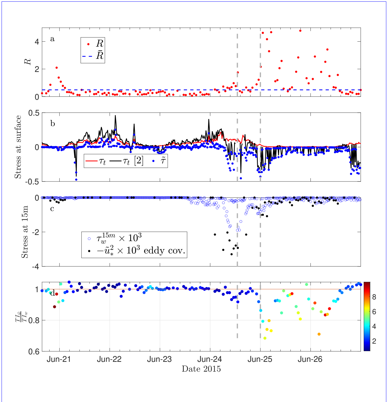
Figure 8. Time series of (a) the wave-turbulence strength ratio R ; (b) momentum stresses at the surface calculated using COARE 3.6 algorithm (red line), Donelan et al. (1999) parameterization Eq. (11), black line, and the wave-induced momentum flux estimated from Eq. (12); and (c) the momentum fluxes at 15 m height estimated using decomposed turbulent wind data based on eddy covariance technique and the estimated wave-induced stress at the same height using Eq. (12) for z = 15 m; and (d) the ratio of the wave induced turbulence intensity, TI_w / TI_w .
