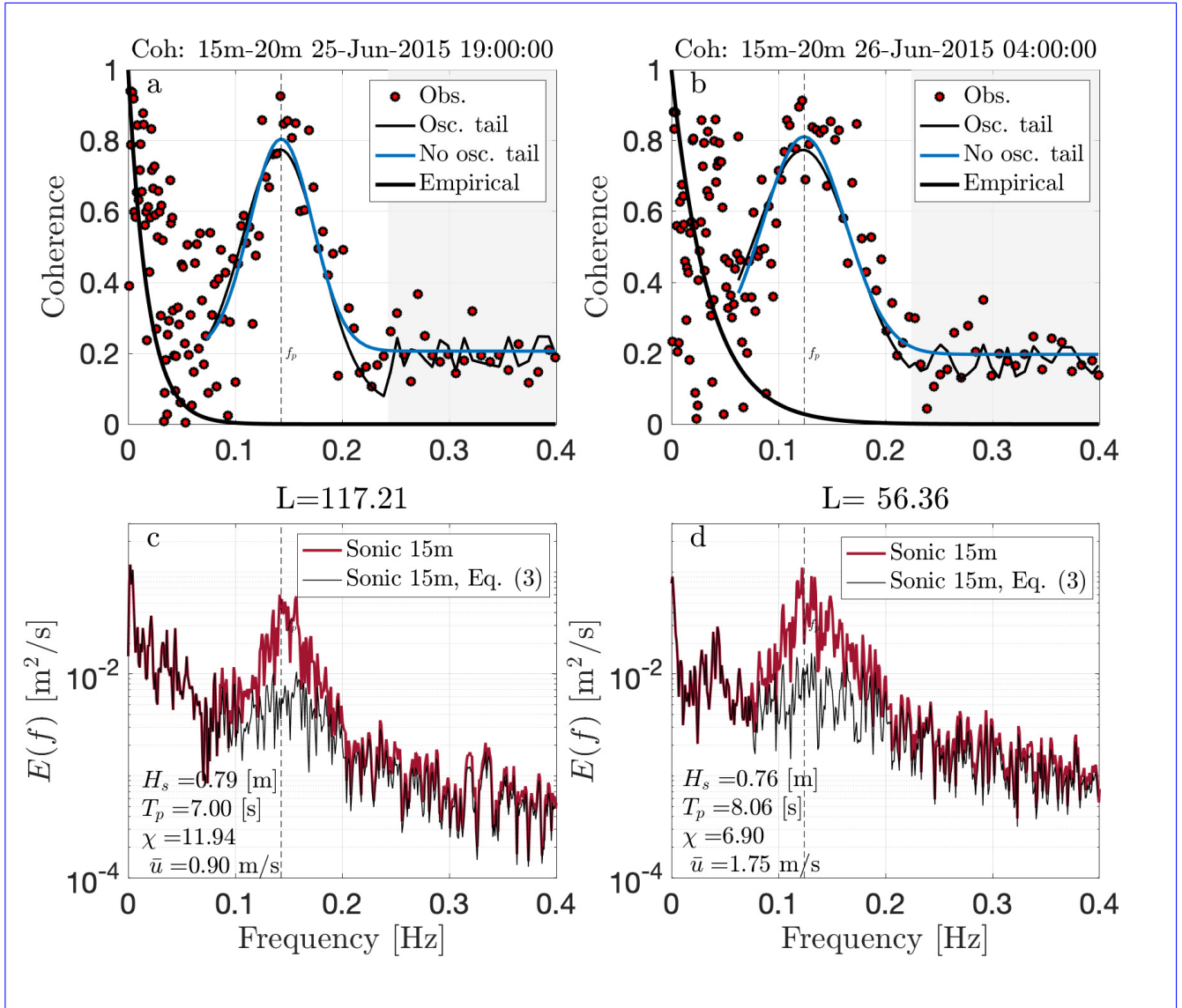
Figure 4. (a,b) The coherence spectra of vertical velocity time series at two heights (15 m and 20 m) are marked in red. In these plots, the thick black curves represent the empirical/theoretical coherence function, while the black thin and blue curves represent the fitted coherence derived from Eq. (2). The black thin curves illustrate the impact of wave-induced oscillations in the coherence tail (shaded regions); and (c,d) power spectra of the original vertical velocity fluctuations for two distinct dates during stable atmospheric conditions, depicted by the red curves. The black curves represent the spectra of turbulent components obtained directly through the coherence-based correction based on Eq. (3).
