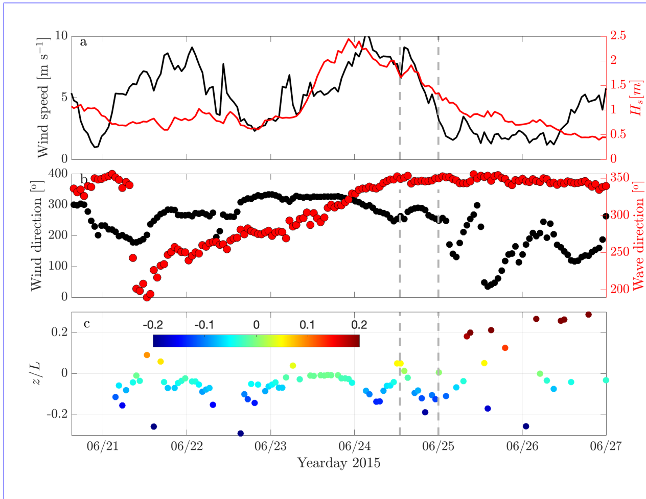
Figure 2. (a) Times series of wind speed at 10 m height measured by the FINO1’s cup anemometer (black line) and significant wave height (red line) measured by a floating buoy operating in the close vicinity of FINO1 platform; (b) wind (black markers) and wave (red markers); and (c) values of the Obukhov length, L , calculated from sonic measurement at height of 15 m above the mean sea level collected with sampling frequency of 25 Hz between 21 and 27 June 2015. The stability classes have been color-coded in this figure. Vertical grey dashed lines highlight the study events of wind-wave interaction at 24 th June at 13:00 and 25 th June at 00:00, respectively.
