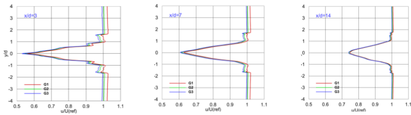
Figure 10. Vertical profiles of the time-averaged normalized x-velocity at different locations downstream of the turbine.
