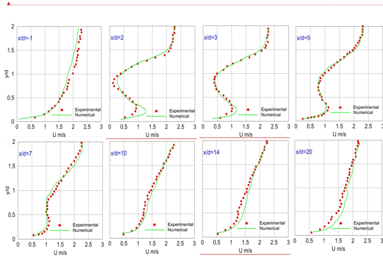
Figure 13. Comparison of vertical profiles of the time-averaged streamwise velocity U ( \text{m s}^{-1} ): ADM-LES (solid line), wind-tunnel measurements (dotted line).
