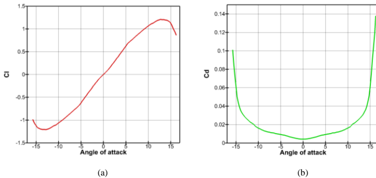
Figure 20. (a) lift coefficient (b) drag coefficient versus angle of attack in 7 \text{ m s}^{-1} wind speed
