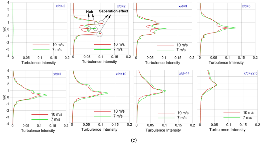
Figure 17. Comparison of vertical profiles of the time-averaged turbulence intensity for one upstream and seven downstream locations for -4 < y/d < 4 at z=0 in \theta_{tilt} = (a) 0^\circ (b) 5^\circ (c) 10^\circ .
