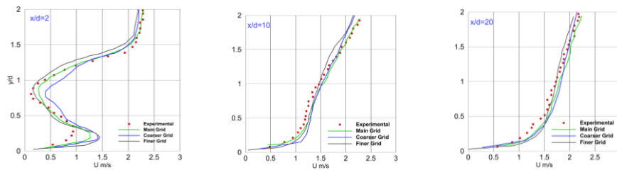
Figure 14. Comparison of vertical profiles of the time-averaged streamwise velocity U ( \text{m s}^{-1} ) obtained by the experiment and different grids.
