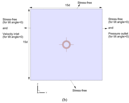
Figure 5. Size of the computational domain and boundary conditions by looking at (a) x-y plane (b) z-y plane
