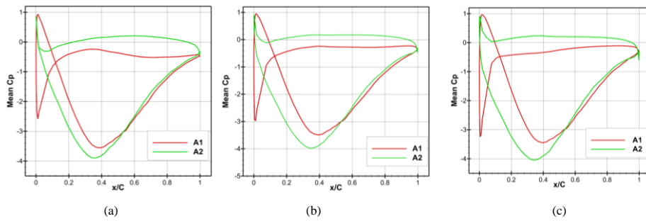
Figure 23. Mean C_p for A1 and A2 airfoils in streamwise direction for U_{ref} = 7 \text{ m s}^{-1} and \theta_{tilt} = 10^\circ in (a) \beta = 30^\circ , (b) \beta = 45^\circ and (c) \beta = 60^\circ .
