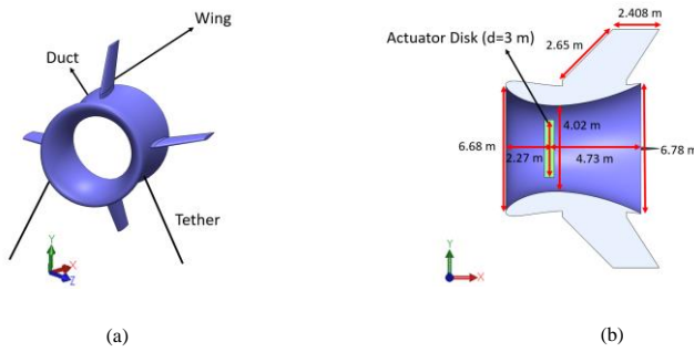
Figure 3. (a) the 3D model of the balloon with a duct (NACA 9415 airfoil cross-section) and 4 wings (n0009sm-ii airfoil cross-section), (b) Geomatic dimensions of the balloon and AD position inside it.
