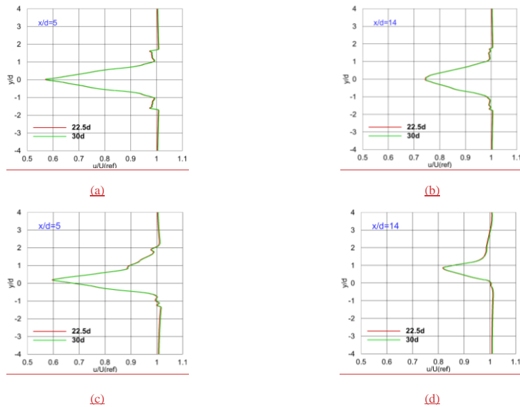
Figure 75. Comparison of vertical profiles of the time-averaged normalized x-velocity for different downstream lengths for U_{ref}=7 \text{ m s}^{-1} , -4 < y/d < 4 , and z=0 with \theta_{tilt}=0^\circ at (a) x/d=5 (b) x/d=14 and \theta_{tilt}=10^\circ at (c) x/d=5 (d) x/d=14 .
