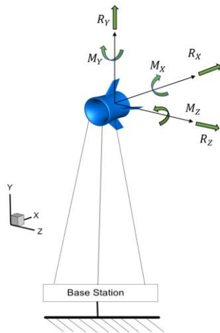
Figure 2018. A schematic of aerodynamic loads on the balloon.
