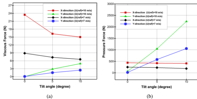
Figure 2119. (a) viscous forces and (b) pressure forces on balloon in the x and y directions variation with wind speeds and tilt angles.
