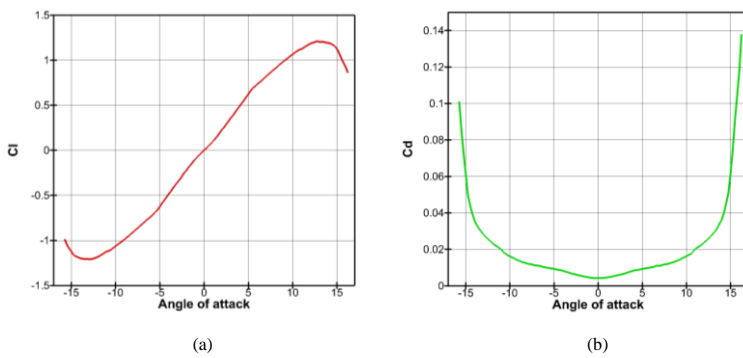
Figure 220. (a) lift coefficient (b) drag coefficient versus angle of attack in 7 \text{ m s}^{-1} wind speed.
