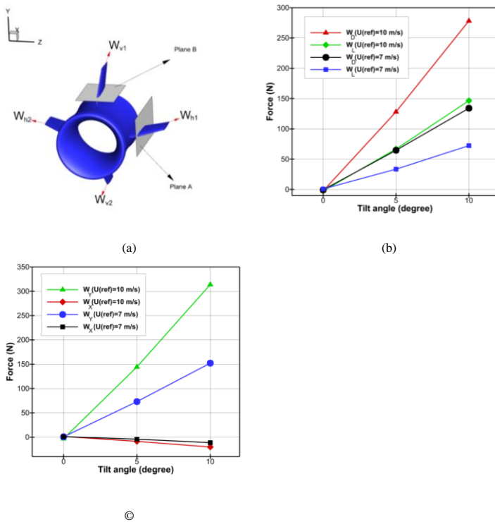
Figure 2321. (a) wings' names (b) lift and drag forces on wing W_{h1} (c) projection of the corresponding forces in the x and y directions in different wind scenarios.
