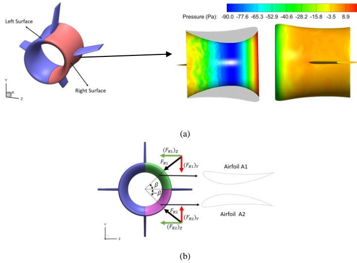
Figure 24.22. (a) pressure contour on the inner and outer surfaces of the right surface of the duct in U_{ref} = 7 \text{ m s}^{-1} and \theta_{tilt} = 0^\circ (b) schematic of the resultant forces on two separate airfoils in different circumferential positions on the duct ( -\beta and \beta around x-axis).
