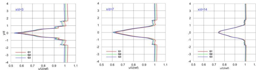
Figure 1210. Vertical profiles of the time-averaged normalized x-velocity at different locations downstream of the turbine.
