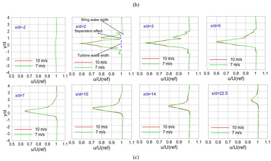
Figure 1715. Comparison of vertical profiles of the time-averaged normalized x-velocity for one upstream and seven downstream locations for -4 < y/d < 4 at z=0 in \theta_{tilt} = (a) 0^\circ (b) 5^\circ (c) 10^\circ .
