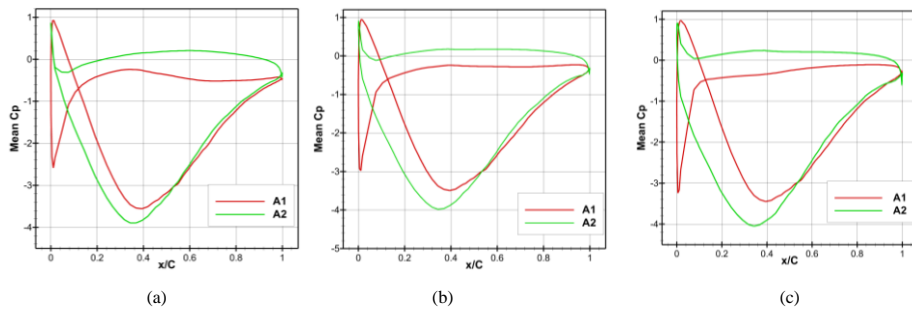
Figure 25.23. Mean C_p for A1 and A2 airfoils in streamwise direction for U_{ref} = 7 \text{ m s}^{-1} and \theta_{tilt} = 10^\circ in (a) \beta = 30^\circ , (b) \beta = 45^\circ and (c) \beta = 60^\circ .
