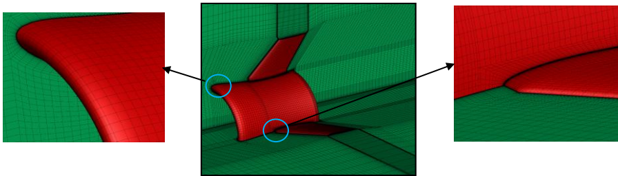
Figure 1344. Mesh distribution on the balloon body, two perpendicular planes passing through, and an exaggerated view of mesh in the boundary layers of one wing and the duct.
