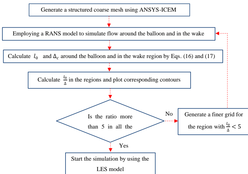
Figure 108. The steps in generating mesh to resolve 80% of total TKE around the balloon and in the wake.
