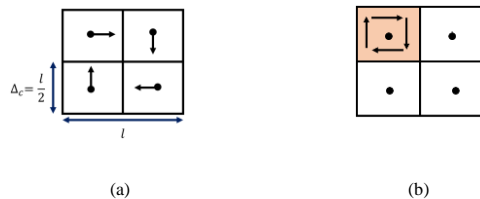
Figure 86. Cells size around a (a) resolved eddy, (b) modeled eddy.
