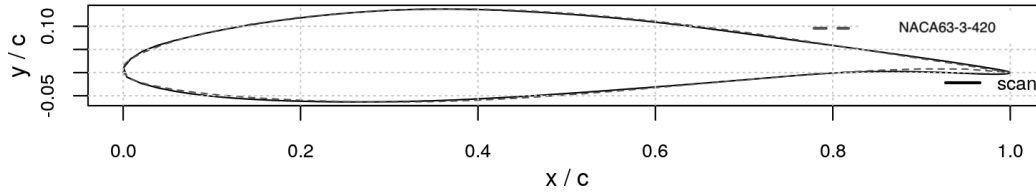
Figure 7. Blade section at 82% of the radius in comparison with a NACA63-3-420 profile with a modified camber of 4% instead of 2% (from Neunaber et al. (2022); published under CC BY-NC-ND 4.0 (License)).
