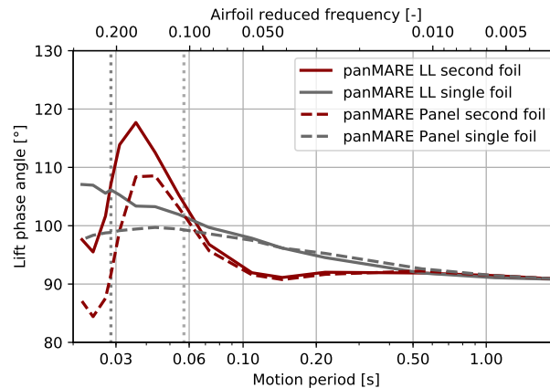
Figure 16. Phase shift between lift and surge position correspiong corresponding to amplitudes of two-dimensional simulations shown in Figure 14.
