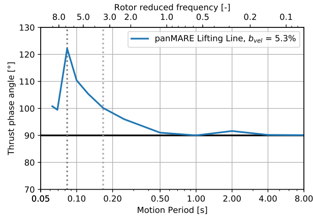
Figure 18. Phase shift between rotor thrust and surge position correspieng corresponding to amplitudes of the UN-AFLOW rotor shown in Figure 17.
