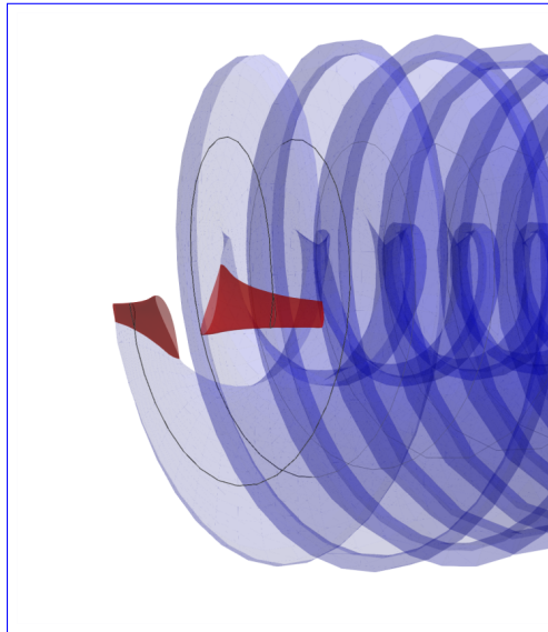
Figure 2. Illustration of blades and wake of the TUHH rotor as modelled in the panel method. A sectional view of blades and wake at a relative radius of 62% is shown in black.
