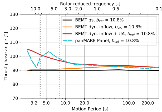
Figure 21. Phase shift between rotor thrust and surge position correspieng corresponding to amplitudes of the IEA 15 MW rotor shown in Figure 19.
