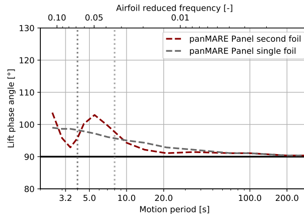
Figure 22. Phase shift between lift and surge position correspieng corresponding to amplitudes of two-dimensional simulations shown in Figure 20.
