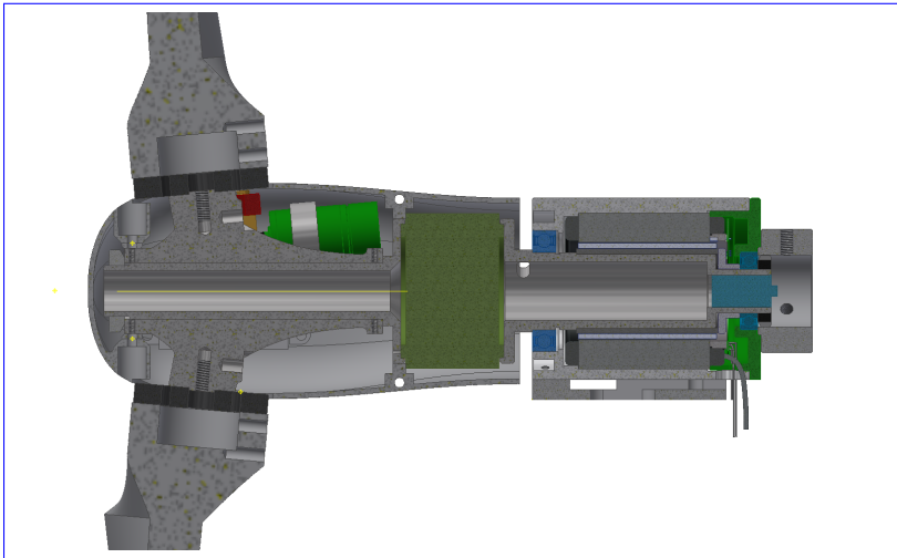
Figure C1. Sectional view of the nacelle. The load sensor (dark grey) is illustrated in dark grey and the main bearings are coloured green.
