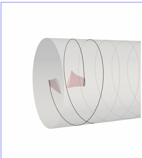
Figure 2. Illustration of blades and wake of the TUHH rotor as modelled in the panel method. A sectional view of blades and wake at a relative radius of 62% is shown in black.
