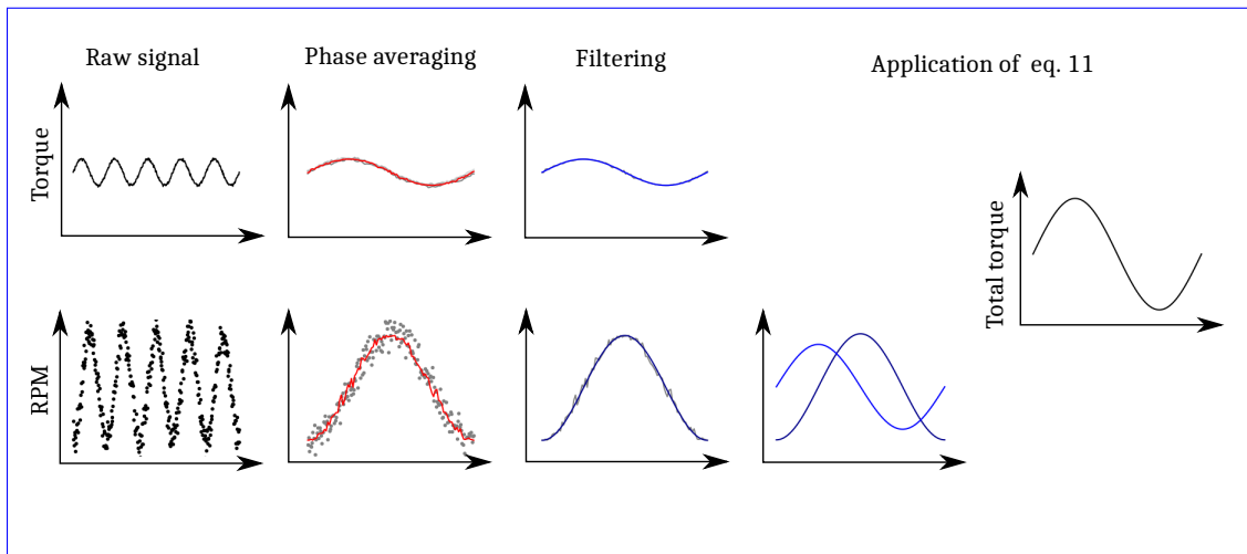
Figure C2. Illustration of the processing steps for rotor torque measurement from load sensor measurements.
