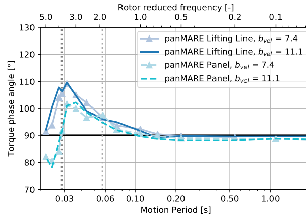
Figure 15. Phase shift between rotor torque and surge position correspiong corresponding to amplitudes of the model rotor shown in Figure 11.
