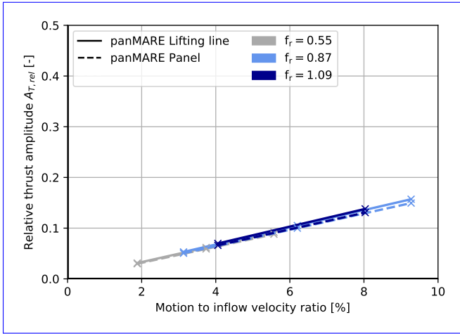
Figure 6. Simulated rotor thrust amplitudes as response to the surge motions ratio. Values are normalised according to equation 12.
