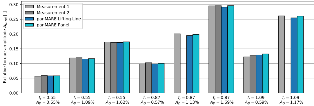
Figure 8. Measured and simulated relative rotor torque amplitudes as response to 8 different surge motions. Values are normalised by the corresponding average rotor torque without motion according to equation 14 . Two measurement runs under identical conditions are shown for most surge motions. A_D describes the motion amplitude normalised to the rotor diameter.
