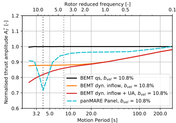
Figure 19. Calculated rotor thrust amplitudes of the IEA 15 MW as a response to surge motions plotted over motion period and rotor reduced frequency. Thrust amplitudes A_T^* are normalised to the scenario-case with the highest motion period ( compare equation 15 ) in case of the panel method and to the quasi-steady simulation in case of the BEMT.
