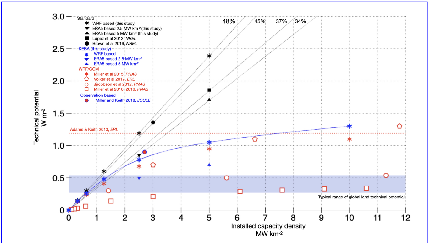
Figure 5. Technical potentials per unit surface area plotted against the capacity density and number of turbines (x-axis). Black symbols represent standard estimates (No-KE removal), while red symbols represent meteorological estimates with WRF or climate models (With-KE removal). Blue symbols represent the KEBA estimates from this study. ERA-5 based estimates are represented separately with upward (5 MW km -2 ) and downward (2.5 MW km -2 ) facing triangles. The blue band represents the range of average peak global potentials (Miller et al., 2011; Jacobson and Archer, 2012; Miller and Kleidon, 2016; Marvel et al., 2012; Wang and Prinn, 2010, 2011; Gustavson, 1979). The red dotted line represents the peak average potential of Kansas (Adams and Keith, 2013) while the dotted lines show the assumed capacity factors estimated without accounting for the removal of KE. Existing estimates of the Kansas resource potential are shown in black filled symbols (Brown et al., 2016; Lopez et al., 2012) (?Lopez et al., 2012). The red circle with the blue outline shows an observation-based estimate (Miller and Keith, 2018).
