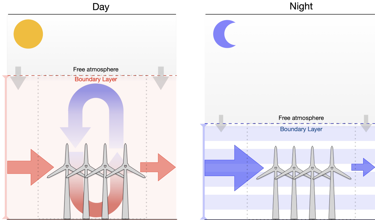
Figure 2. Differences between daytime (left) and nighttime (right) boundary layer conditions Gray downward arrows represent and their effect on the downward flux renewal of kinetic energy from the free atmosphere into the boundary layer (grey arrows) and convective mixing (blue/red arrow in left panel). The red and blue arrows represent the horizontal kinetic energy in- and outflow (from left to right) through the boundary layer volume bounding the regional scale wind turbine deployment (dotted box) during day and night, respectively. The free atmosphere represents the part of the atmosphere in which large-scale motion is generated in the absence of friction.
