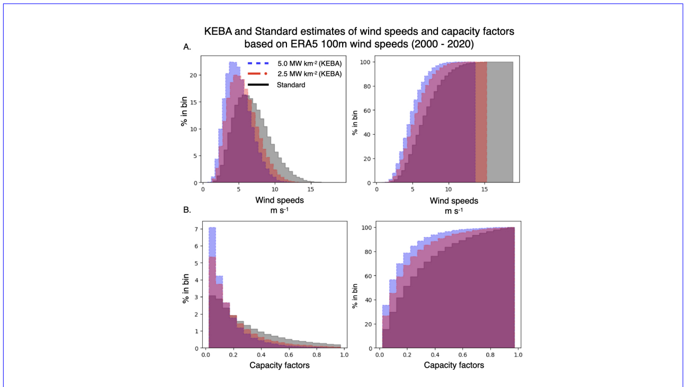
Figure E2. Wind speed (A) and capacity factor (B) distributions for standard and KEBA approaches for the 2.5 (red) and 5 MW km -2 (blue) deployment scenarios calculated using ERA-5 100m wind speeds over the 2000-2020 period.
