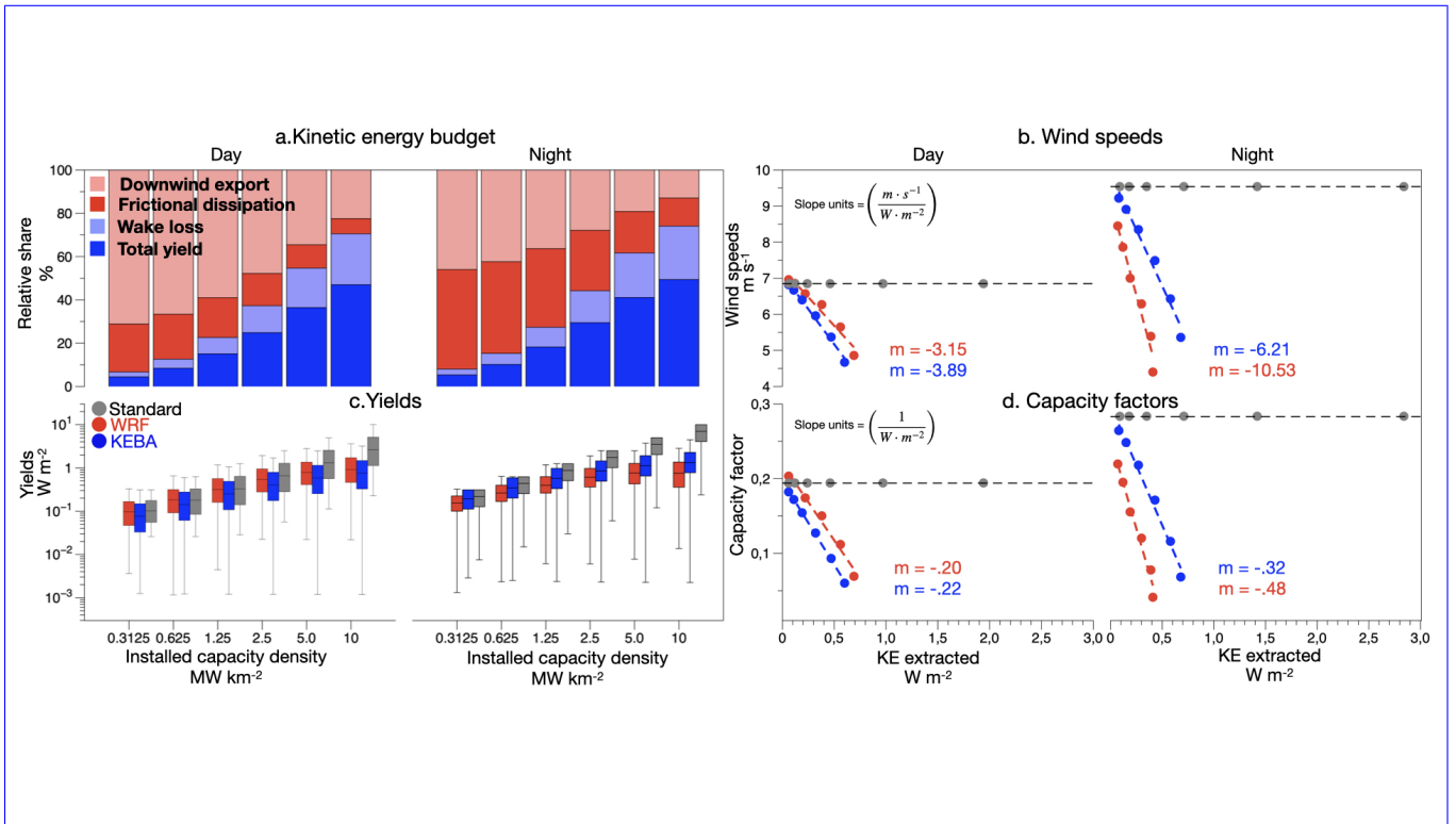
Figure 3. (a) Daytime (left) and nighttime (right) KE budgets, with total yields (dark blue), wake loss (light blue), frictional dissipation (red) and the downwind export (light red). (b) Estimates of wind speeds over the deployment region against the KE extracted by the wind turbines for the "standard" (grey), "WRF" (red) and "KEBA" (blue) estimates. (c) Wind turbine yields as a function of installed capacity density using a logarithmic scale for the "standard" (grey), "WRF" (red) and "KEBA" (blue) estimates. (d) Capacity factors against the rate of KE extraction for the "standard" (grey), "WRF" (red) and "KEBA" (blue) estimates. Dashed lines in (b) and (d) denote linear fits. m denotes the slopes obtained from linear regression. The units for the slope in (b) and (d) are (m \cdot s^{-1})(W \cdot m^{-2})^{-1} and (W \cdot m^{-2})^{-1} , respectively.
