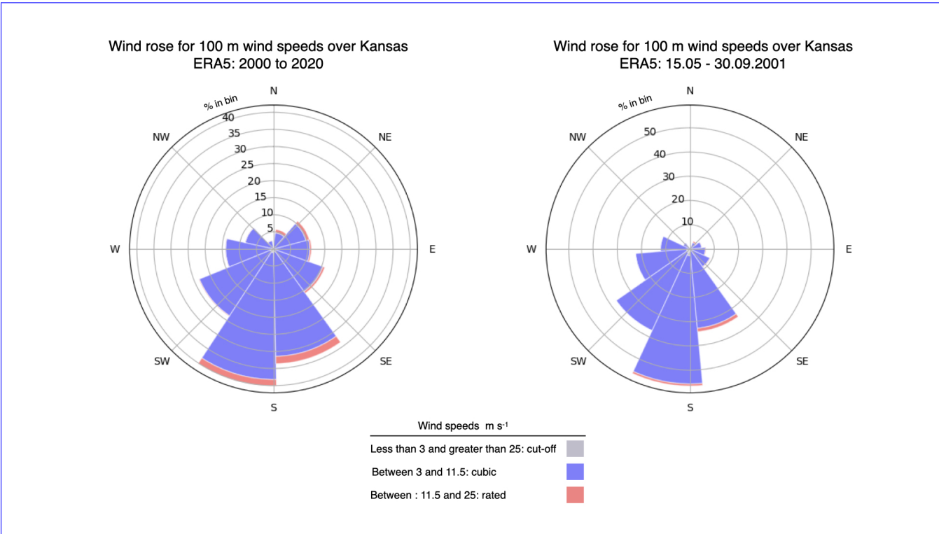
Figure E1. Wind directions for 100m wind speeds over Kansas from ERA-5 over the 2000-2020 period.
