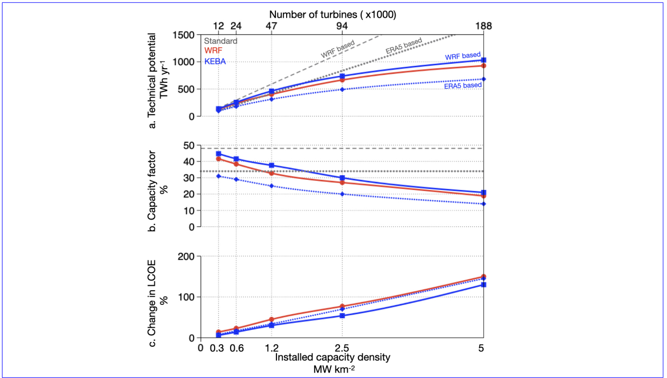
Figure 6. (a.) Variation in WRF (red ○) KEBA (blue □ with solid line, blue ◇ with dotted line) and standard (gray stippled and dotted lines) estimates of technical potential, (b.) capacity factors, and (c.) % change in the Levelised Cost of Energy (LCOE) relative to the standard LCOE estimate plotted as a function of capacity densities (bottom) and number of turbines deployed (top). Standard and KEBA estimates based on WRF Control and ERA-5 data have been represented separately.
