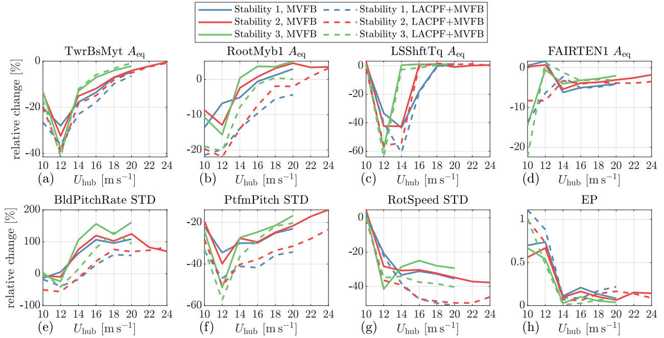
Figure 10. Relative changes of equivalent load amplitudes, standard deviations, and energy productions under different mean wind speeds. The relative changes are calculated using the values by optimally tuned MVFB and LACPF+MVFB controllers relative to that by the MVFB controller with baseline tuning .
