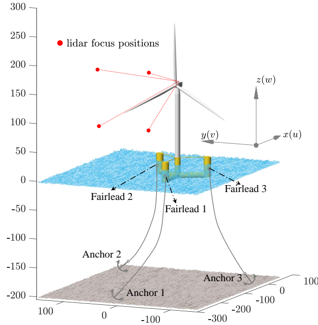
Figure 1. A sketch of the investigated IEA 15MW reference turbine equipped with a four-beam nacelle lidar system and UMaine semi-submersible floating platform, drawn using the CAD data provided by the IEA Wind Task 37 GitHub repository. The coordinate system follows right hand rule (with a unit in m) and is applicable to the full paper. Note that the positions of the anchors are not true values due to the limitations of the figure frame.
