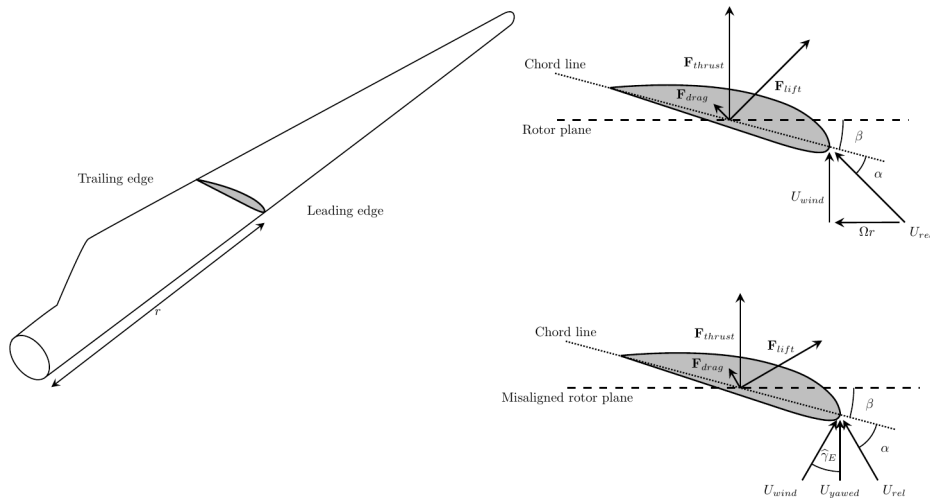
Figure 4. Blade element dynamics under normal and yawed conditions, \hat{\gamma}_E = \gamma_E \sin(\theta) and U_{yawed} = U_{wind} \cos(\hat{\gamma}_E) . Illustration adapted from Howland et al. (2020).
