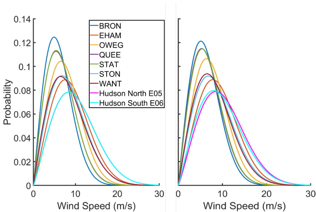
320 Figure 4. Probability distributions from the Weibull fits to 10-minute wind speeds at 150 m height from the NYSERDA LiDAR buoys and the NYSM stations for all available data (left) and year with common highest data availability ('best year' of September 2018-2019) (right). Note: probability distributions from Hudson North E05 and Hudson South E06 virtually overlay each other in the left panel.
