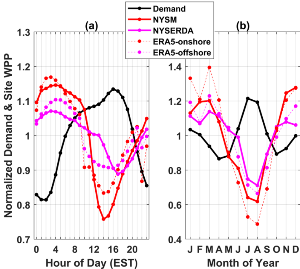
450 Figure 9. Normalized (a) diurnal and (b) monthly cycles of electricity demand for New York State (black) and wind power production (WPP) at NYSM (red) and NYSERDA (magenta) sites. ERA5-derived WPP is shown for the grid-cells which contain the NYSM and NYSERDA LiDARs (thin, dashed lines) for the climatological period, 1979-2022. The data are normalized to a mean value of 1 and so that values of 0.9 or 1.1 in a given hour or month indicates WPP or demand that is 10% below or above the mean, respectively.
