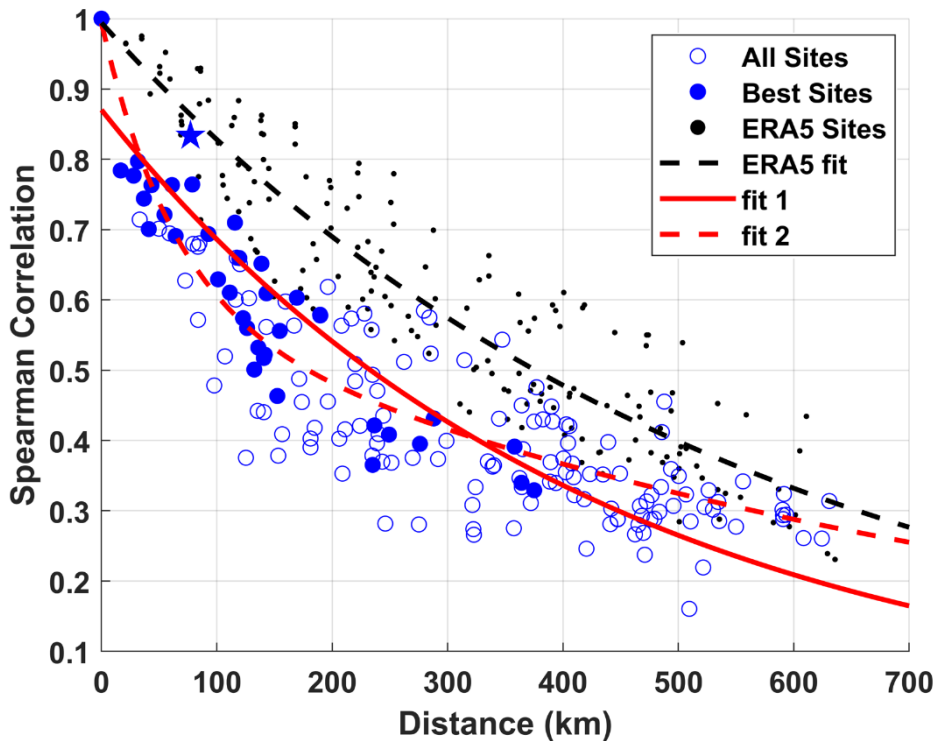
390 Figure 7. Spearman spatial correlation coefficient ( r ) of power production for the LiDAR (blue) and ERA5 (black) output sampled at the NYSEERDA and NYSM locations against the separation distance between all 19 sites (17 onshore, 2 offshore). Solid blue points indicate location pairs with high data availability, open points represent the relationships including the remaining NYSM sites. The star represents the correlation between the two NYSEERDA buoys. Best fit lines ( y = Spearman correlation coefficient, x = spherical 395 distance between locations) are shown for the LiDAR: y = 0.8703\exp(-0.002377x) (solid red) and y = 0.4021\exp(-0.01595x) + 0.5914\exp(-0.0012x) (dashed red). The fit to the ERA5 estimates has the form y = 0.9942\exp(-0.00183x) (dashed black).
