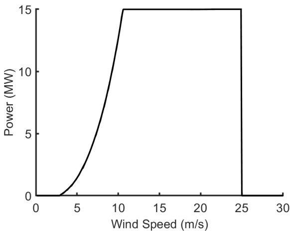
205 Figure 2. Power curve for the IEA 15 MW reference wind turbine (Gaertner et al., 2020).
