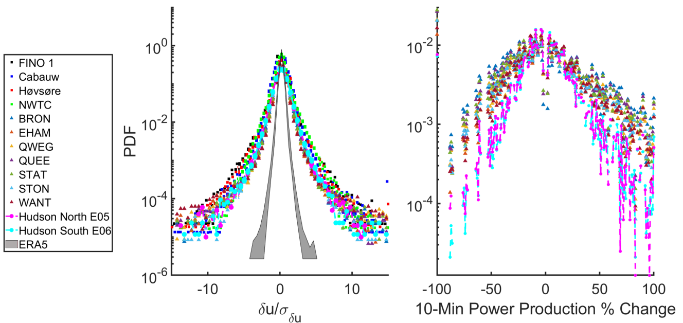
355 Figure 5. Left: probabilities of wind speed ramp events computed from the 10-minute data from the NYSERDA LiDAR buoys and the NYSM sites computed using Equation (3), and reported for four locations at or near operating wind turbines: FINO 1 is (offshore) in the North Sea, Cabauw is in the western portion of the Netherlands, Høvsøre is in Jutland, Denmark, and NWTC is in the foothills of the Colorado Rocky Mountains (data digitized from: (DeMarco and Basu, 2018)). Wind ramps computed from the hourly ERA5 output are shown by the gray polygon. Right: probabilities of wind power production ramp events at the locations of the NYSERDA buoys and the NYSM sites computed by applying the power curve for the IEA 15 MW reference wind turbine to the LiDAR wind speeds. The probabilities of no-change (i.e., power \pm 0\% ) are not shown to aid visibility.
