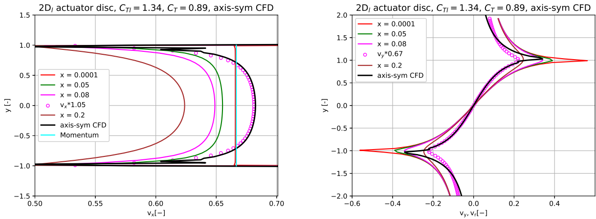
Figure 6. The graph to the left is a zoom of the right graph in Fig. 5. In the right graph 2D l v_y velocity profiles are compared with the radial velocity profile from an axis-symmetric simulation. At the same downstream position x = 0.08 as for the v_x component the best fit for v_y is obtained with a scaling factor of 0.67.
