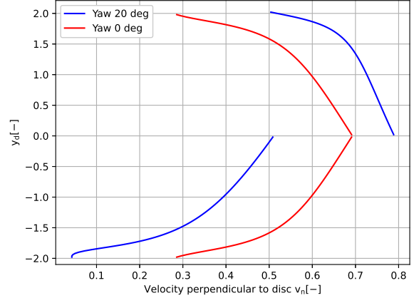
2D l actuator disc, coning 30 deg, yaw 20 deg, C_{Tl} = 1.34 , C_T = 0.89
