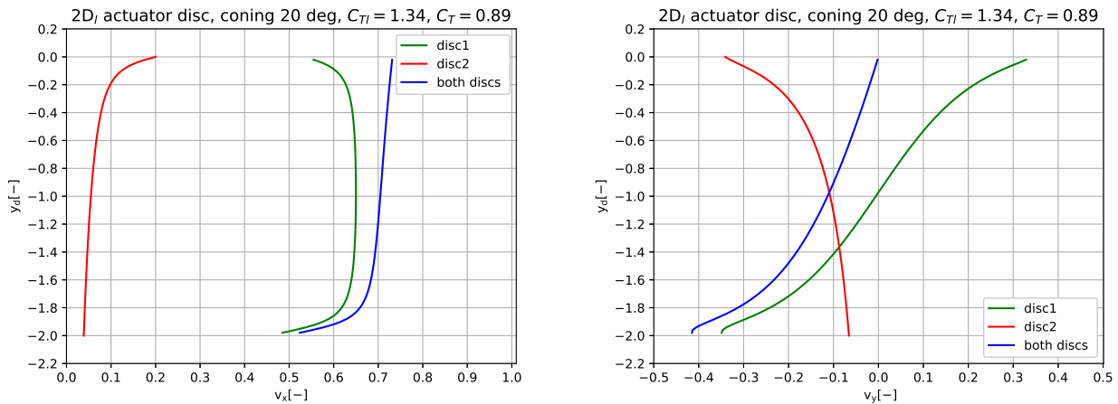
Figure 14. In the left graph we show the v_x components contributing to the total induction on the lower part, disc 1. The same for v_y in the graph to the right.
