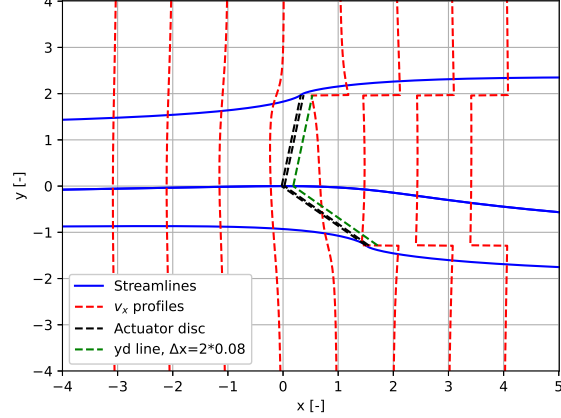
2D l actuator disc, coning 30 deg, yaw 20 deg, C_{Tl} = 1.34 , C_T = 0.89
