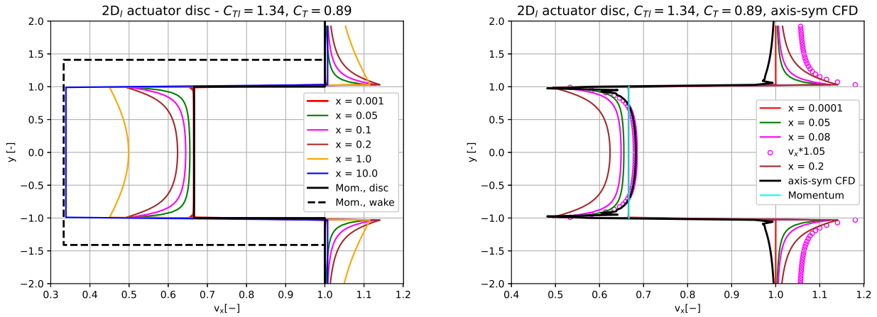
Figure 5. In the left graph we show the axial velocity v_x profiles at positions close behind the disc as well as further downstream for a thrust coefficient of 0.89. For comparison the momentum solution for v_x at the disc and in the far wake is also included. In the graph to the right the v_x velocity profile at the disc from an axis-symmetric CFD AD simulation is compared with the 2D l profile at a downstream distance of 0.08 scaled with factor 1.05 to account for the decrease of velocity downstream behind the disc and to give the best fit to the CFD results extracted at the disc.
