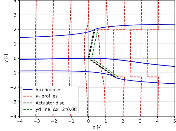
2D I actuator disc, coning 30 deg, yaw 20 deg, C_{Tl} = 1.34 , C_T = 0.89
