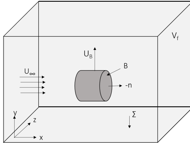
Figure 1. Schematic representation of a fluid domain containing a cylindrical rigid body.
