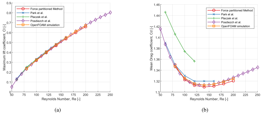
Figure 5. Variation of (a) maximum lift coefficient and (b) mean drag coefficient for a fixed cylinder at different sub-critical Reynolds numbers compared against literature: citepPark1998, Placzek et al. (2009) and Posdziech and Grundmann (2007).
