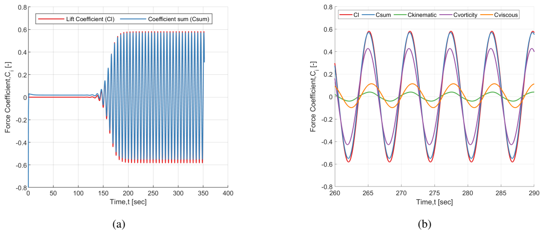
Figure 7. (a) Comparison of lift force coefficient against the sum of force coefficients from the force-partitioning method. (b) A zoomed-in snippet is shown, which breaks down the total force coefficient into partitioned force coefficients.
