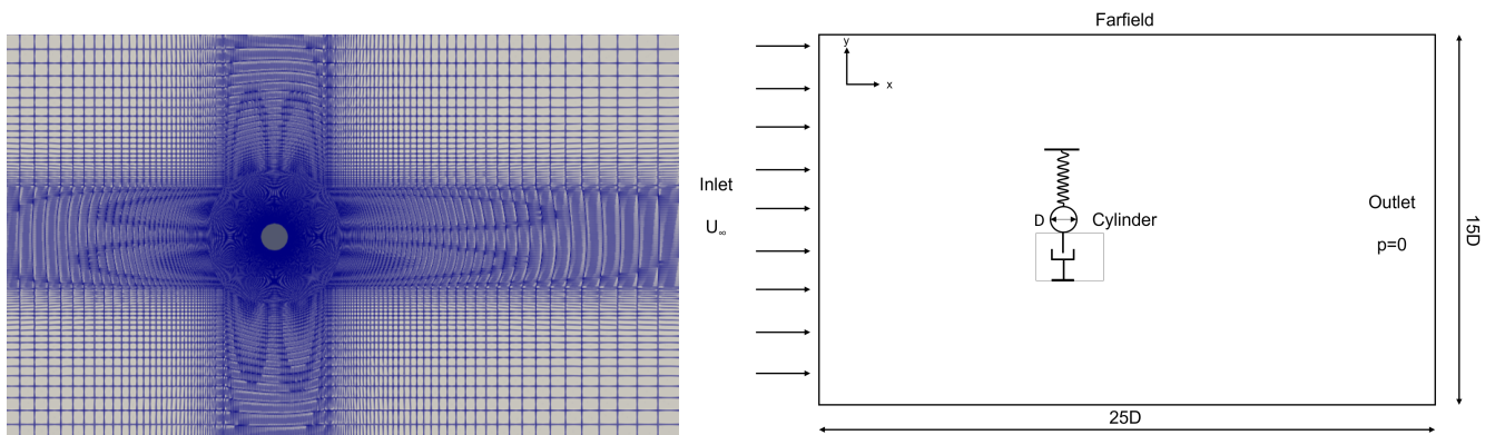
Figure 3. Schematic representation of the computational domain: Cartesian mesh (left), domain characteristics (right).
