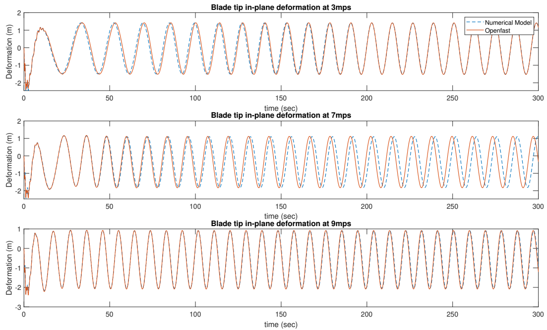
Figure 1. Model Verification: Blade in-plane displacement In-plane deformation response at the blade tip
