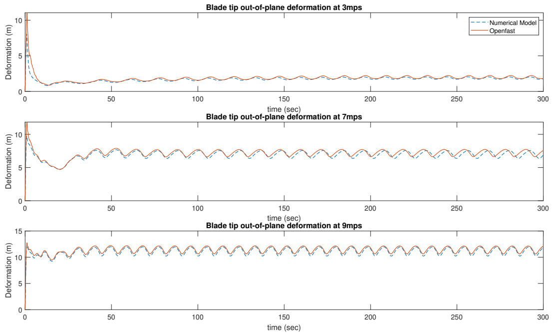
Figure 2. Model Verification: Blade out-of-plane displacement Out-of-plane deformation response at the blade tip
