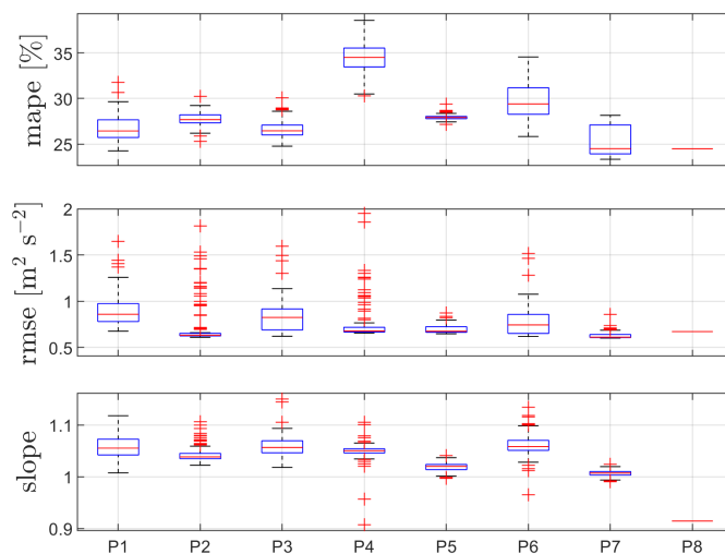
Figure 20. Performance of the DDNNs for different set of inputs P (see Table 2) at 37 m. Box plots of 100 trained datasets
