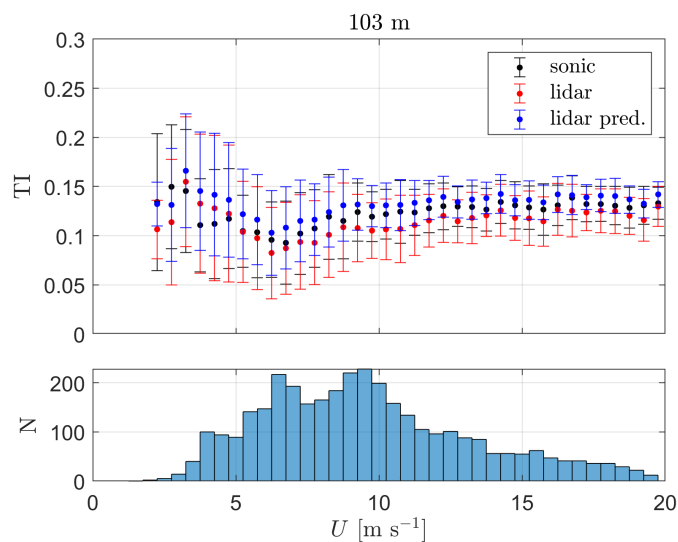
Figure 23. Similar to Fig. 21 but for the 103-m height
