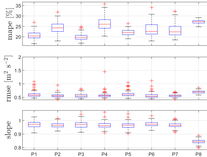
Figure 19. Box plots of the cross-validation for the DDNNs with different set of inputs (see Tab. 2) of 100 randomly tested datasets at 37-m height. Box plot information as in Fig. 10
