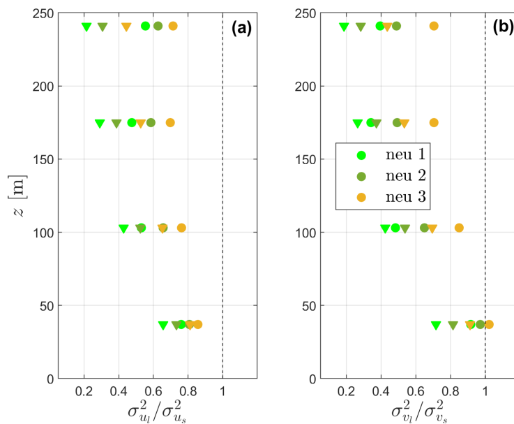
Figure 6. Lidar-to-sonic ratio of the u -variance (a) and v -variance (b) as function of height under neutral atmospheric conditions for the three length-scale categories (Table 3). Model results and measurements are shown in triangles and circles, respectively. Colors are in agreement with those of Fig. 5
