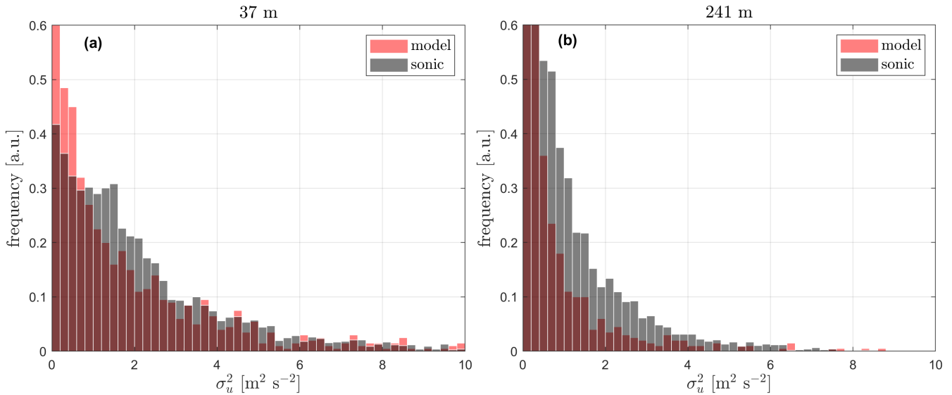
Figure 9. Normalized histograms of the u -variance from the sonic-anemometer measurements and the Mann model-based turbulence climatology at 37 (a) and 241 m (b)
