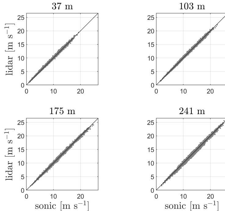
Figure 4. 10-min means of horizontal velocity measured by the sonic anemometers and lidar 1 for each of the matching heights
