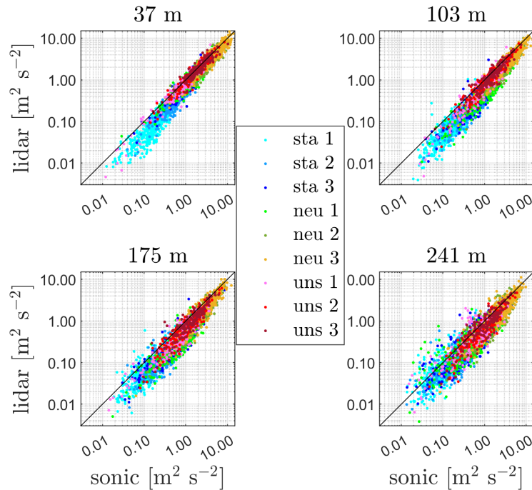
Figure 5. 10-min along-velocity variances measured by the sonic anemometers and lidar 1 for each of the matching heights. The different categories are color-coded and refer to those in Table 3
