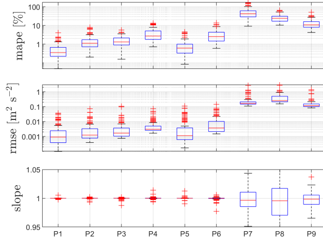
Figure 10. Box plots of the cross-validation for the PBNNs with different sets of inputs (see Table 1) of 100 randomly tested datasets for the height 37 m. Red solid horizontal lines represent medians, blue rectangle limits the 25th and 75th percentiles, whiskers show the maximum and minimum of the range, and red crosses represent outliers
