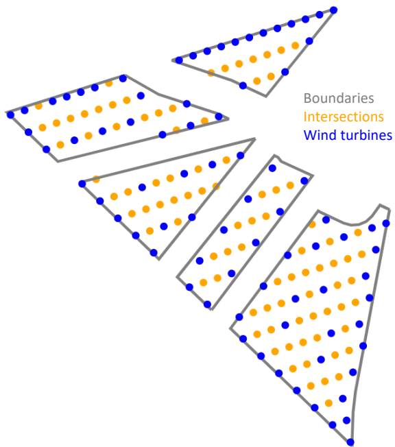
(a) Best 81-turbines wind farm layout
