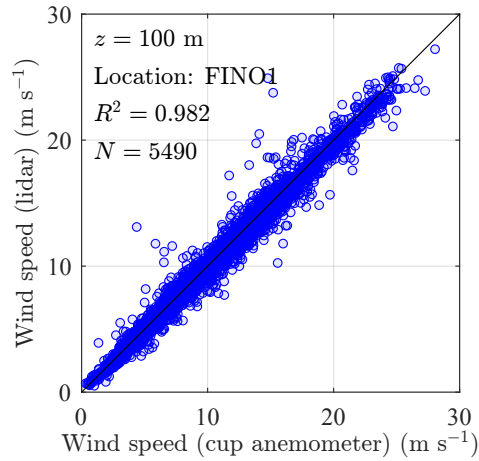
Figure 3. Comparison of 10-minute mean wind speed measurements recorded by the cup anemometer and the WindCube 100S at 100 m above sea level, collected between June 2015 and October 2016 during the OBLEX-F1 campaign at the FINO1 platform (5490 samples).
