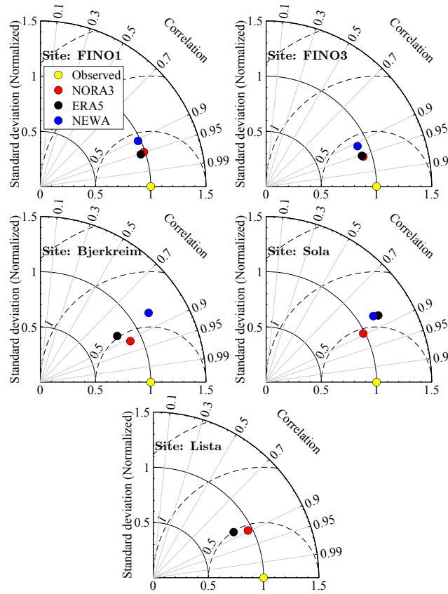
Figure 10. Taylor's diagrams for the five sites at the range gate closest to 150 m: FINO1 ( z = 153 m), FINO3 ( z = 174 m), Bjerkreim ( z = 140 m), Sola ( z = 133 m), and Lista ( z = 100 m).
