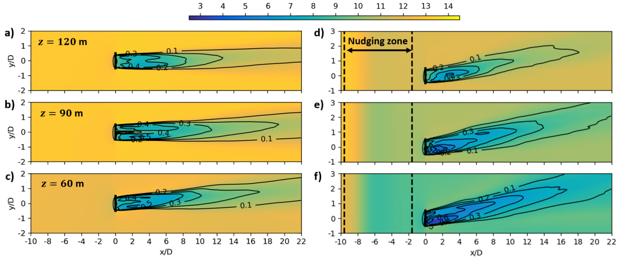
Figure 8. Coloured contours of the time-averaged zonal velocity component \overline{u_{i,j,k}} in \text{m s}^{-1} for SW in a), b) and c) and for SOW in d), e) and f) averaged over 20 min at the end of the simulation. b) and e) show the x - y plane at hub height z = 90 \text{ m} . a) and d) (c and f) correspond to the x - y planes at Z = 90 \text{ m} + R/2 = 120 \text{ m} ( Z = 90 \text{ m} - R/2 = 60 \text{ m} ). The black contours represent the velocity deficit V D_{i,j,k} at the same vertical location calculated in relation to the upstream velocity at x = -200 \text{ m} . The axes are normalized by the rotor diameter D = 126 \text{ m} , whereby x/D = 0 indicates the position of the rotor.
