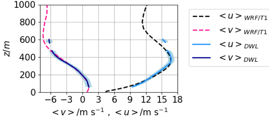
Figure 1. Vertical profiles of the measured velocities at the WiValdi site (zonal \langle u \rangle_{DWL} , meridional \langle v \rangle_{DWL} , shaded areas indicate the DWL uncertainty of \pm 0.5 \text{ m s}^{-1} ) and the continuous profiles from the WRF simulations used as target profile T1 (zonal \langle u \rangle_{WRF/T1} , meridional \langle v \rangle_{WRF/T1} ).
