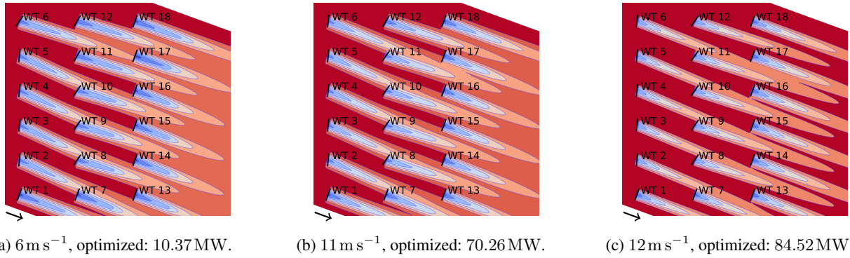
Figure 9. Optimization results for series 3 as shown in Table 7. Subfigure captions specify the wind speed and the farm’s total power output.
