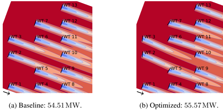
Figure 8. Detailed results for a 6 \times 3 farm in which some turbines are inactive (case 2.5 with wind speed of 11 \text{ m s}^{-1} and direction of 20^\circ ). Subfigure captions specify farm-level yaw control (baseline or optimized) and the resulting total power output of the farm.
