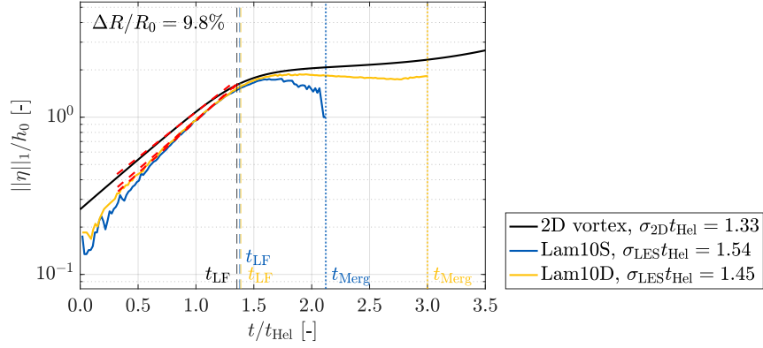
Figure 12. Temporal evolution of \|\eta\|_1 obtained from the LES simulations using the standard mesh (blue line, Lam10S) and the dense mesh (yellow (green) line, Lam10D), alongside the result from the 2D vortex model described in SubSect. 2.5 (black line). The time of the first leapfrogging event (when \beta reaches 90^\circ ) is indicated by t_{LF} , and the time of vortex merging (when b reduces to zero) is marked as t_{Merg} . The growth rates are determined based on the slopes between 0.6 and 0.8t_{LF} , and these slopes are indicated by the red dashed-lines. (We have updated the color scheme to allow the people with color vision deficiencies being able to interpret the figure.)
