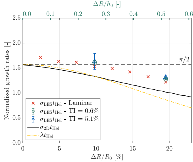
Figure 13. Comparison of growth rates obtained using different methods, including LES simulations with the standard mesh under various in-flow conditions ( \sigma_{LES} ), the 2D vortex model described in SubSect. 2.5 ( \sigma_{2D} ), and the linearized system derived in App. B ( \lambda ). Normalization of these quantities is all against t_{Hel}^{-1} = \Gamma/2h_0^2 . The normalized growth rates \sigma_{LES}t_{Hel} for the two dense-mesh cases with \Delta R/R_0 \simeq 10\% are 1.45 for laminar inflow (Lam10D) and 1.61 for TI = 5.9% (T10D). These values are not plotted to avoid overcrowding the figure. (We have updated the color scheme to allow the people with color vision deficiencies being able to interpret the figure.)
