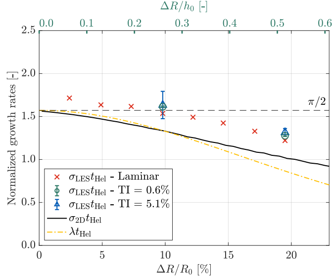
Figure 13. Comparison of growth rates obtained using different methods, including LES simulations with the standard mesh under various inflow conditions ( \sigma_{LES} ), the 2D vortex model described in SubSect. 2.5 ( \sigma_{2D} ), and the linearized system derived in App. B ( \lambda ). Normalization of these quantities is all against t_{Hel}^{-1} = \Gamma/2h_0^2 . The normalized growth rates \sigma_{LES} t_{Hel} for the two dense-mesh cases with \Delta R/R_0 \simeq 10\% are 1.45 for laminar inflow (Lam10D) and 1.61 for TI = 5.9% (T10D). These values are not plotted to avoid overcrowding the figure.
