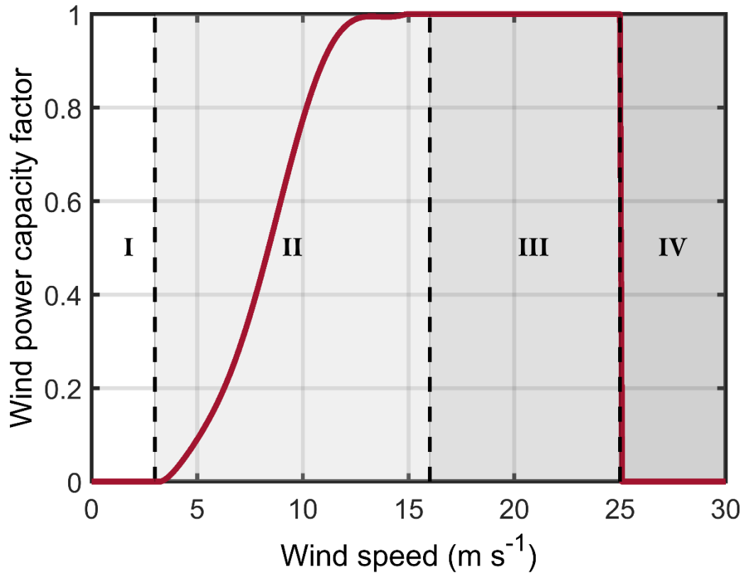
115 Figure 1: Wind speed to wind power capacity factor conversion curve. Cut-in wind speed is 3 \text{ m s}^{-1} and cut-off wind speed is 25 \text{ m s}^{-1} . Regions I, II, III, and IV of the curve are indicated in between the dashed lines.
