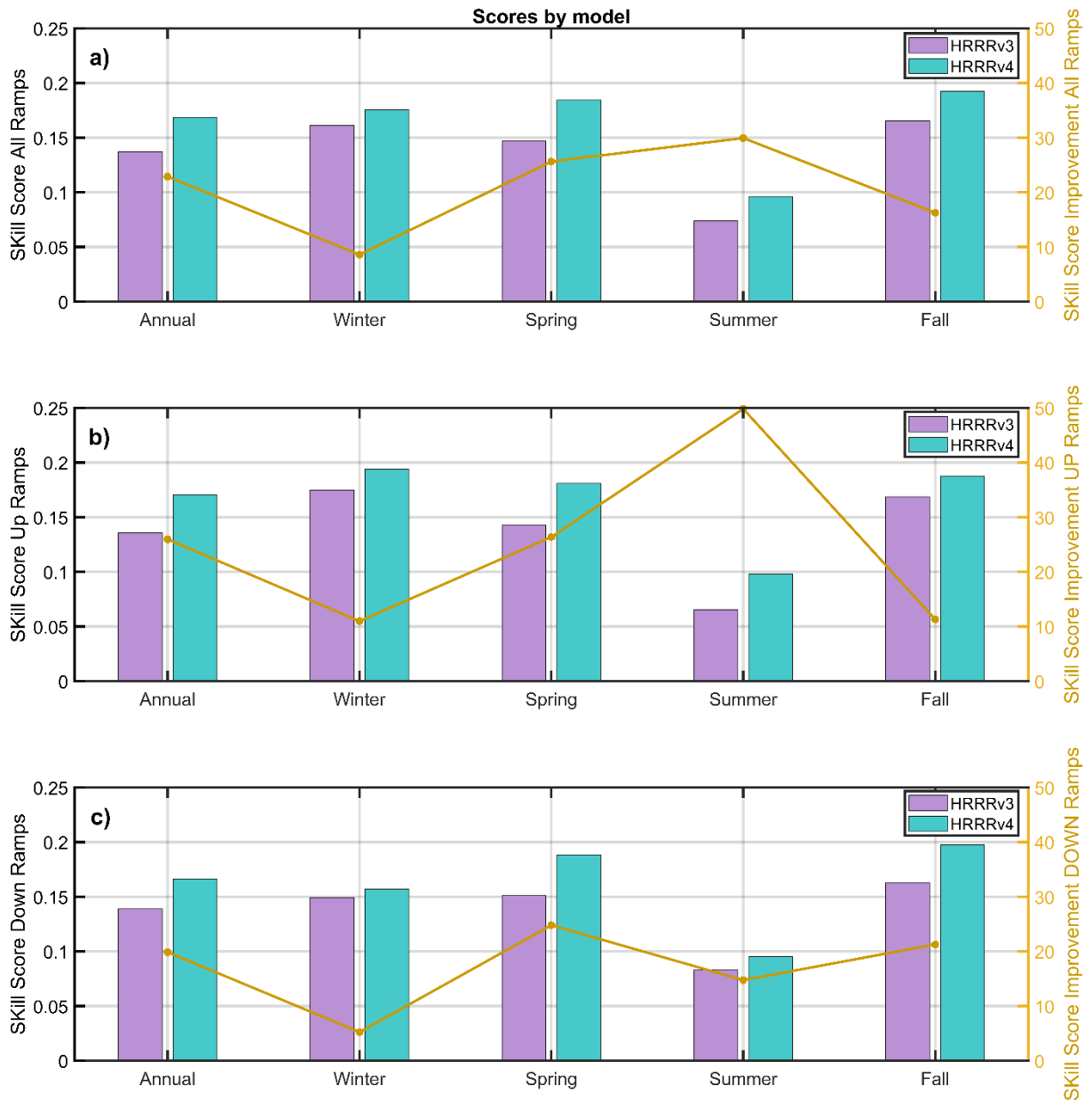
340 Figure 10: Left axes: Bar chart with skill scores averaged by model version annually and by season, for all ramps (panel a), up ramps only (panel b), and down ramps only (panel c). Right axes: Percentage improvements in skill score annually and by season, for all ramps (panel a), up ramps only (panel b), and down ramps only (panel c).
